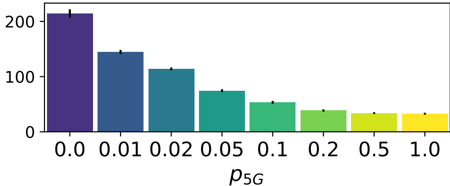
Mean Number of Clusters
