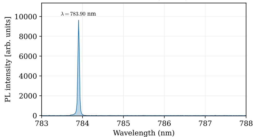
TPE -- exciton X (filtered)
