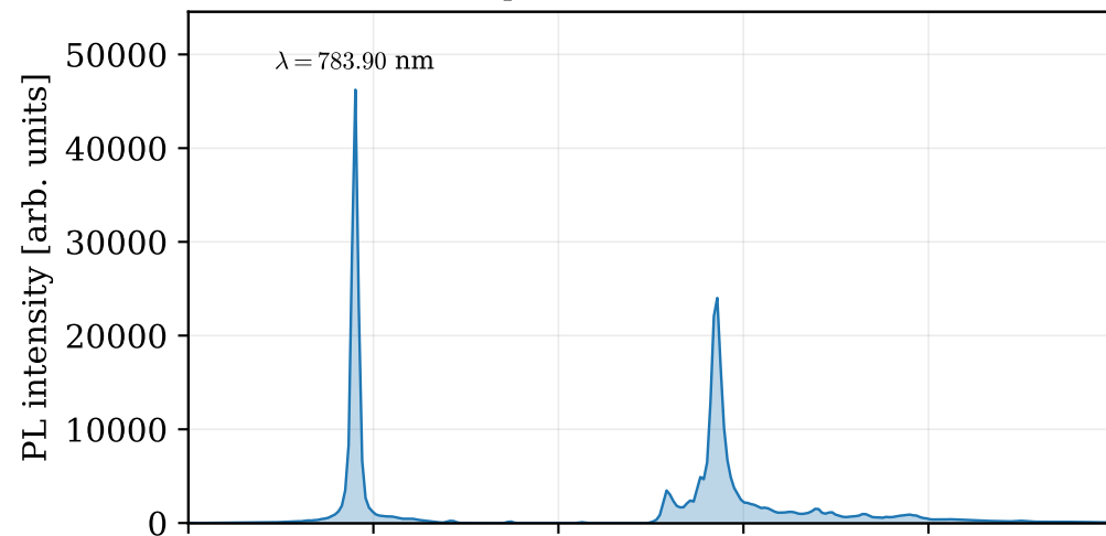
Two-photon excitation (TPE)
