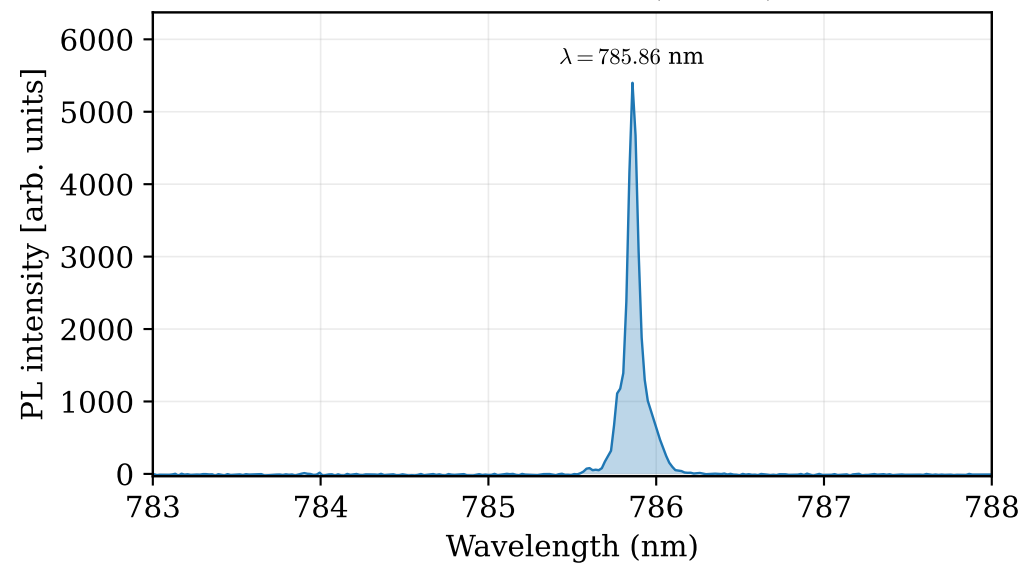
TPE -- biexciton XX (filtered)
