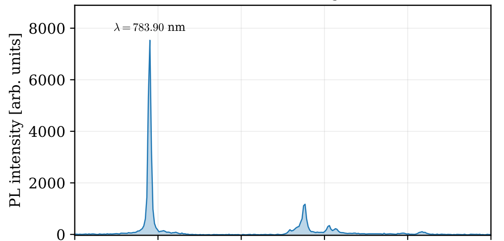
Above-band excitation (green cw)
