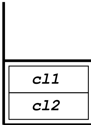
Backtracking stack
