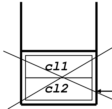
Backtracking stack
