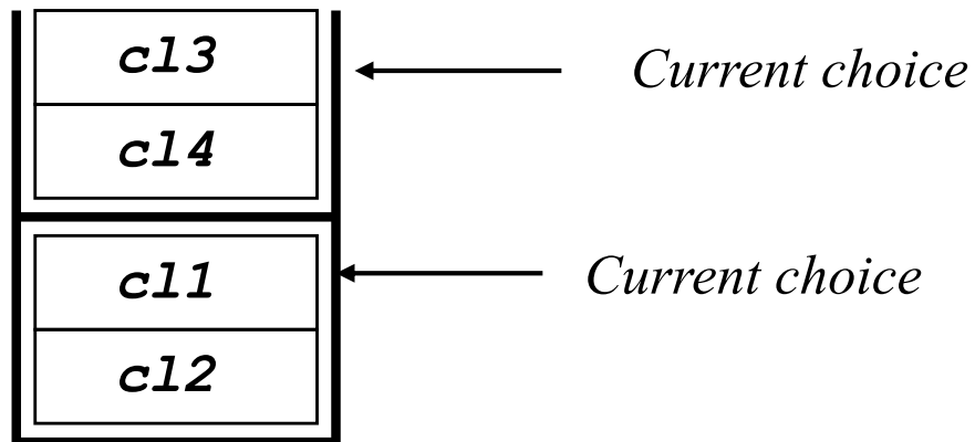
Backtracking stack
