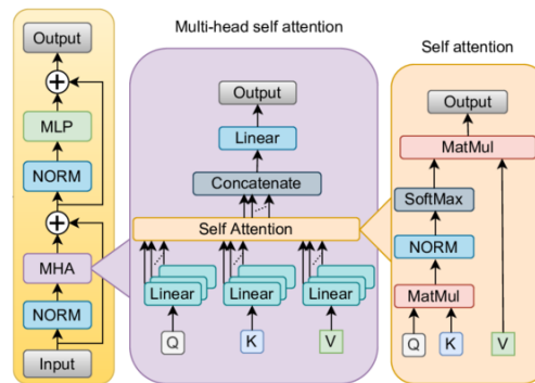
N x transformer block
