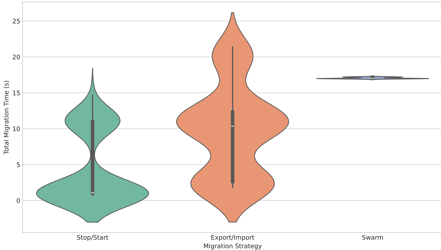
Migration Time Distribution by Strategy
