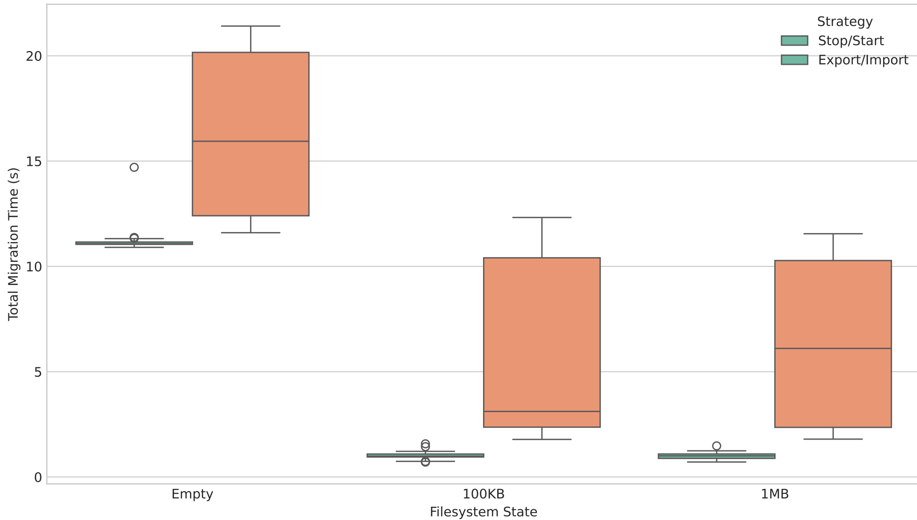
Migration Time by Filesystem State (SSH Strategies)
