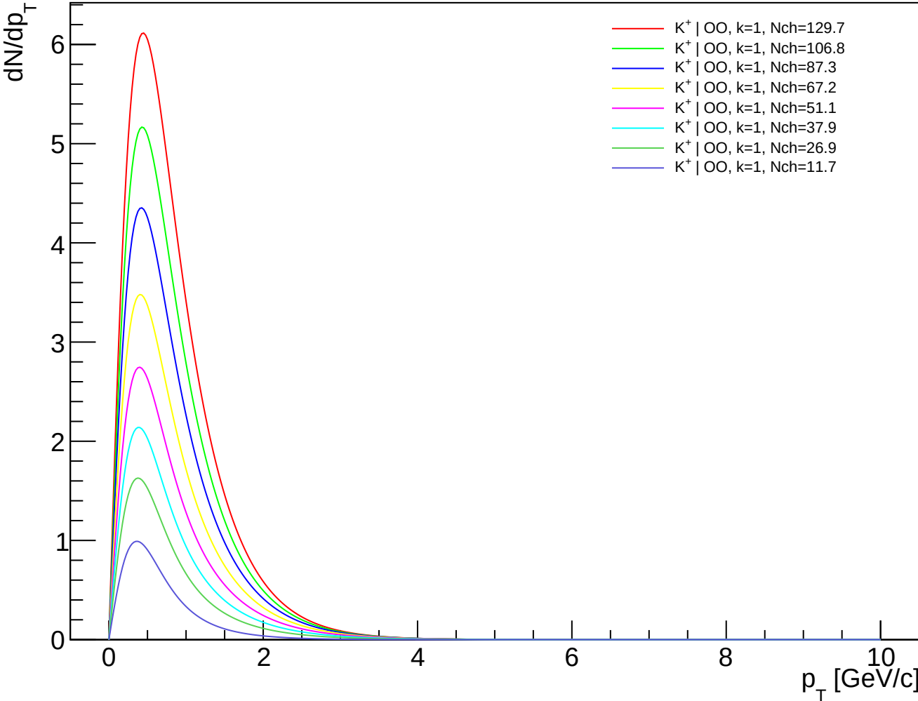
K + (PDG 321) spectra - OO, k=1.00
