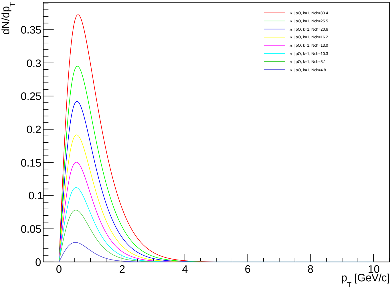
\Lambda (PDG 3122) spectra - pO, k=1.00
