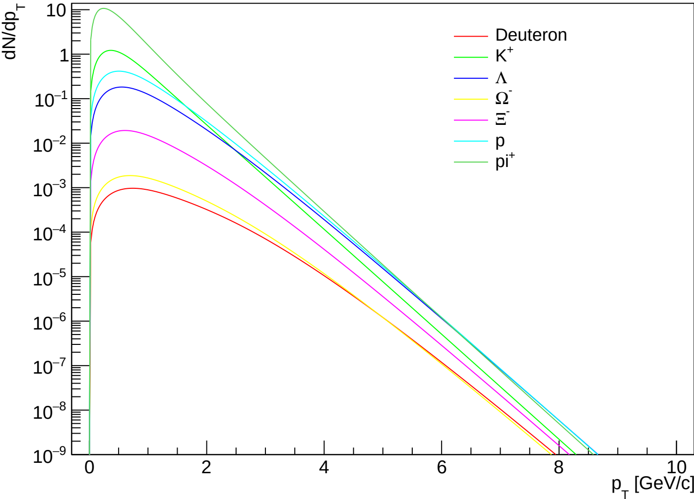
prediction_PbPb5.02_1910.07678_CEGs | k=1.60 | NeNe | cent VIII
