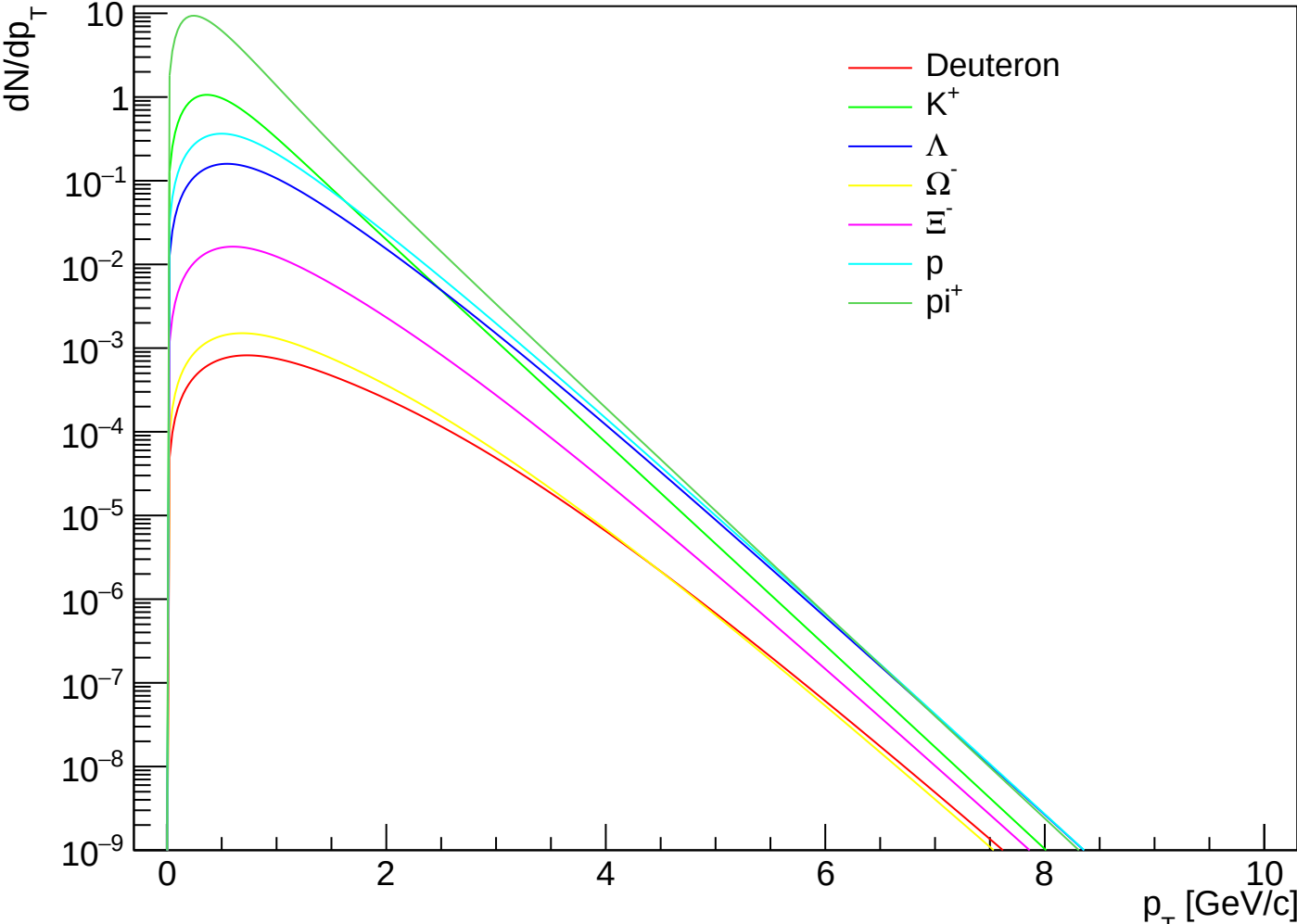
prediction_PbPb5.02_1910.07678_CEGs | k=1.60 | OO | cent VIII
