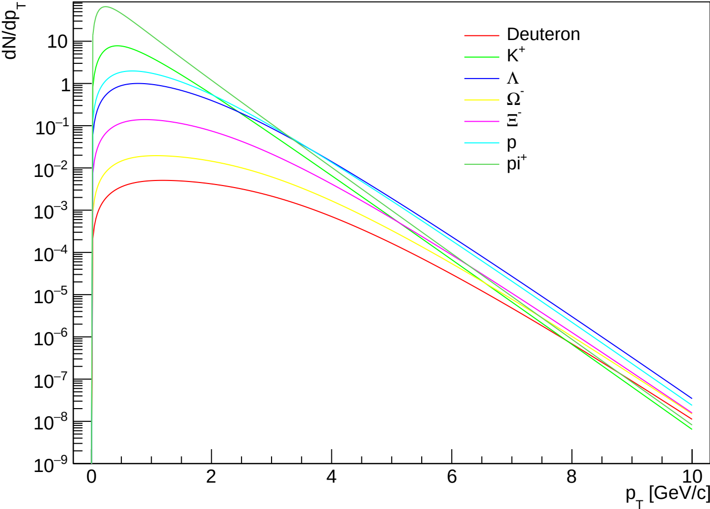
prediction PbPb5.02 1910.07678 CEGs | k=3.00 | OO | cent II
