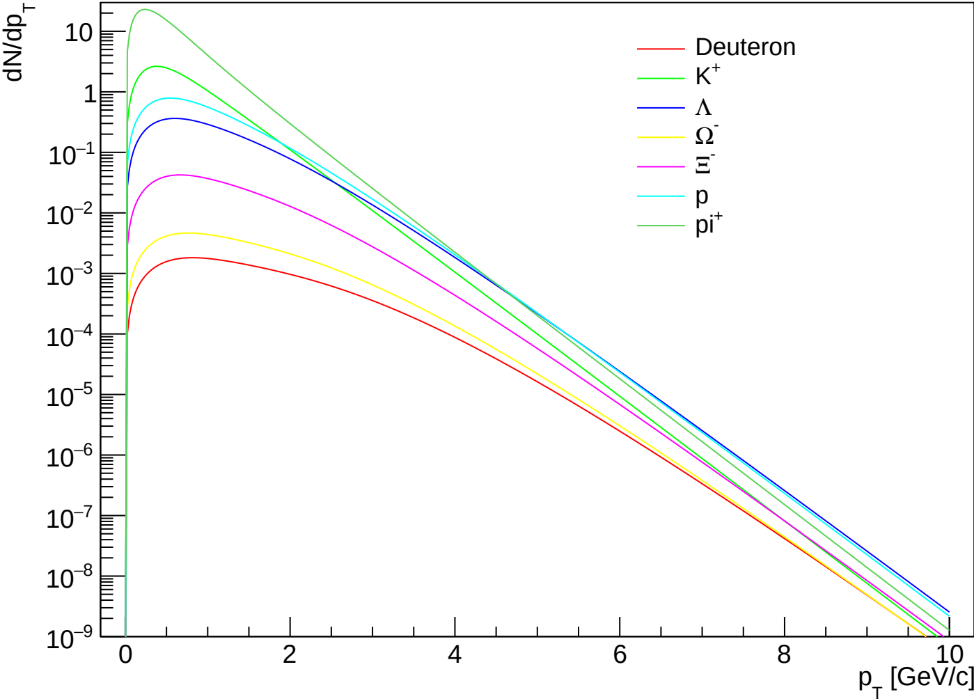
prediction PbPb5.02 1910.07678 CEGs | k=1.00 | NeNe | cent VII
