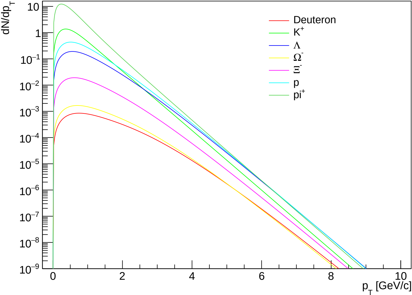
prediction PbPb5.02 1910.07678 CEgs | k=1.00 | pO | cent IV
