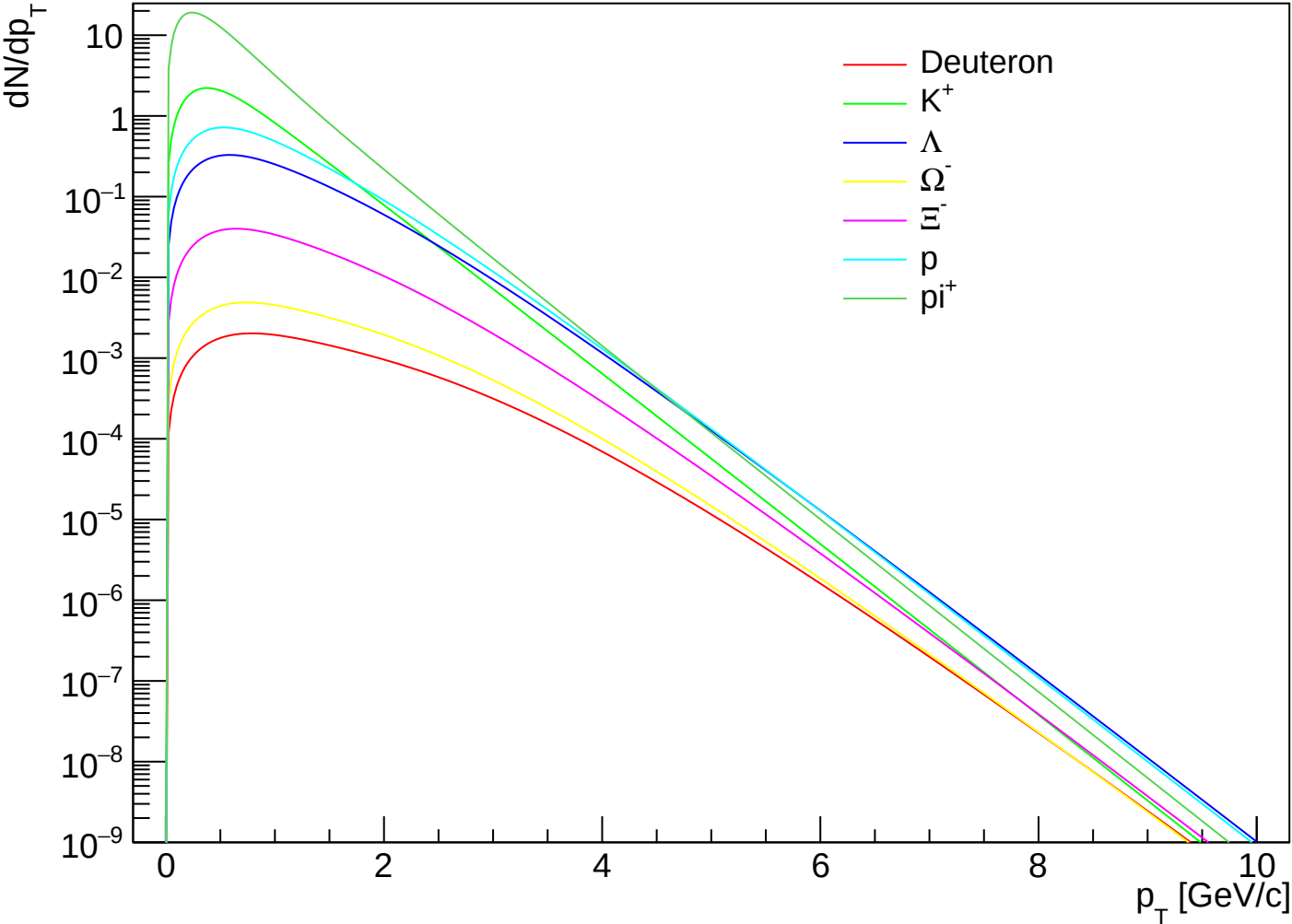
prediction_PbPb5.02_1910.07678_CEGs | k=3.00 | pO | cent II
