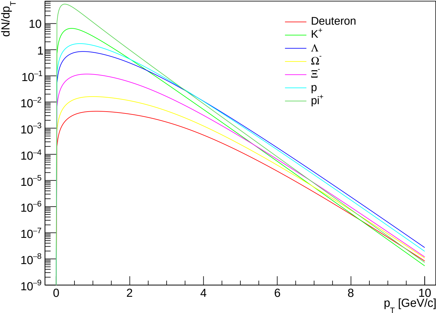
prediction PbPb5.02 1910.07678 CEqs | k=3.00 | OO | cent III
