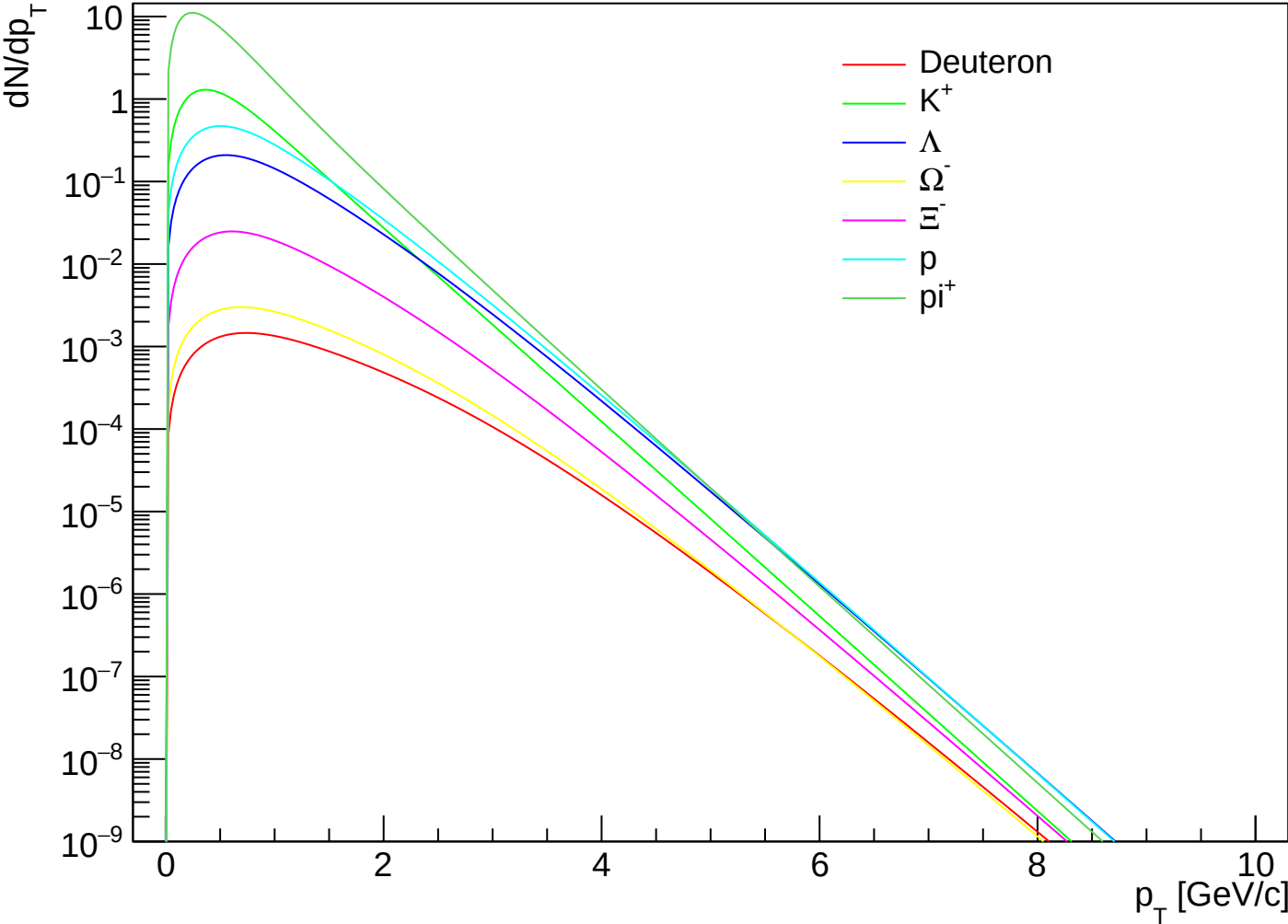
prediction_PbPb5.02_1910.07678_CEGs | k=6.00 | NeNe | cent VIII
