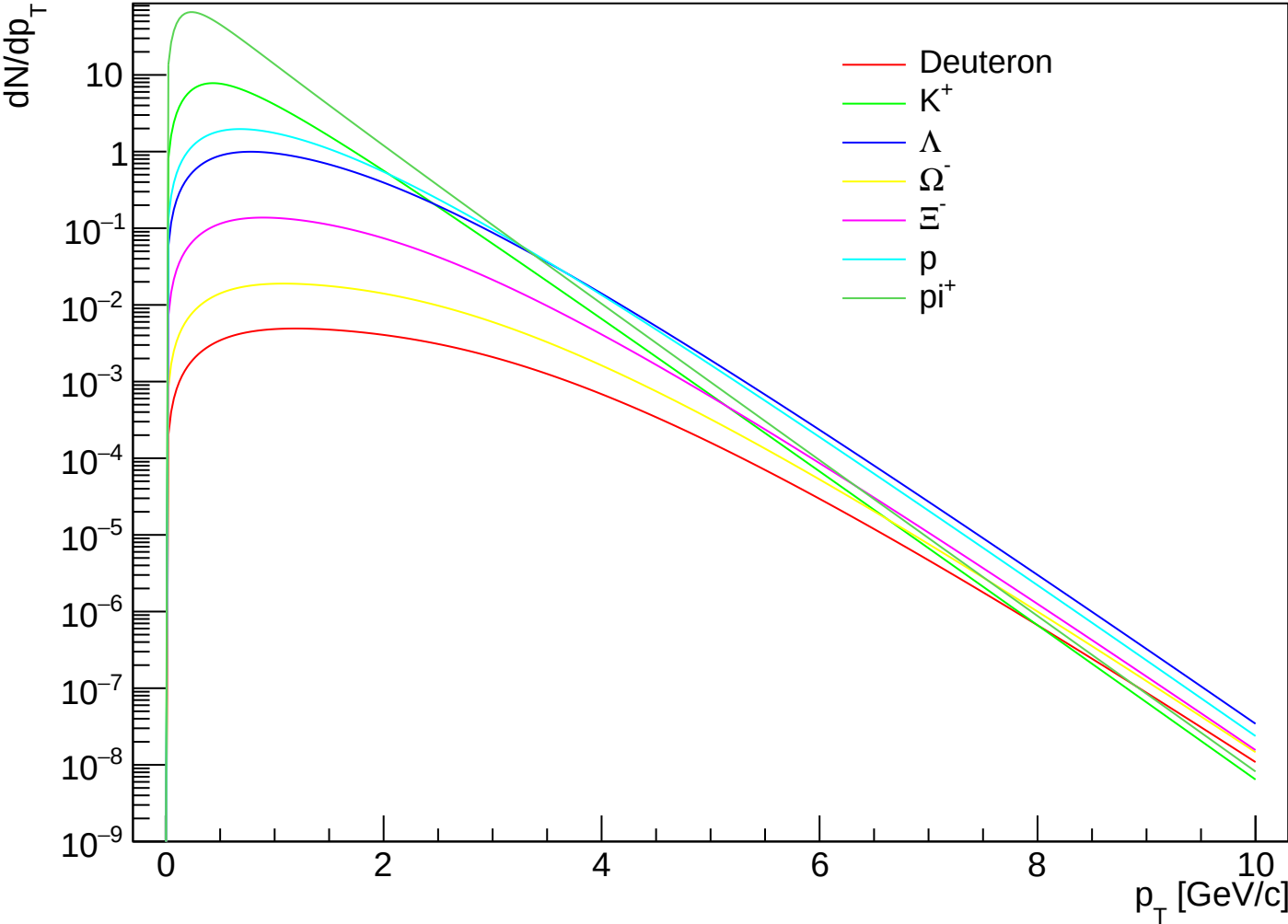
prediction_PbPb5.02_1910.07678_CEGs | k=1.60 | NeNe | cent III
