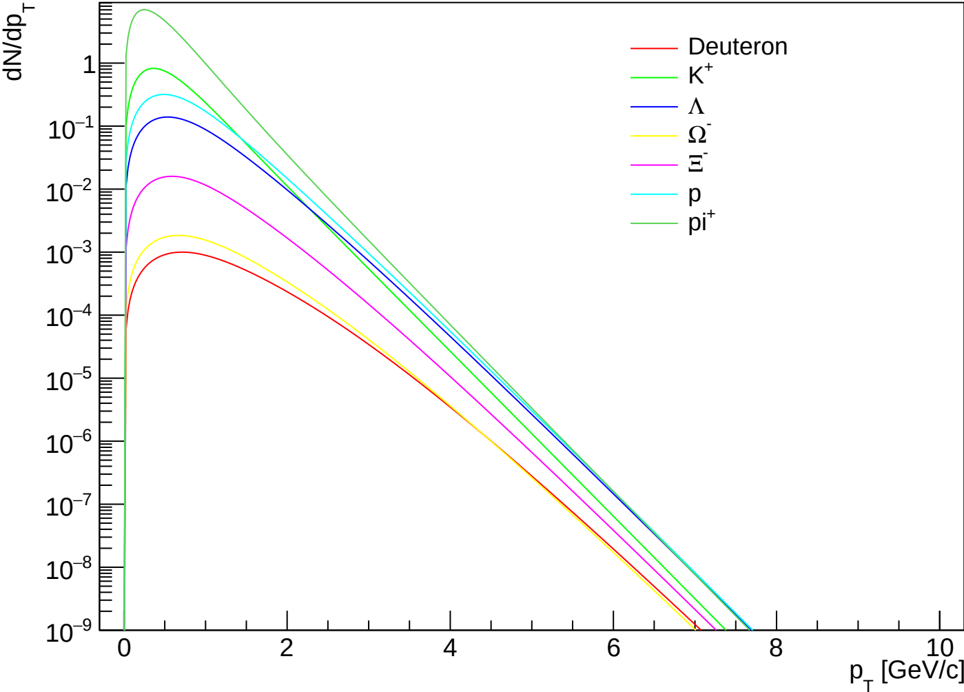
prediction PbPb5.02 1910.07678 CEGs | k=6.00 | pO | cent VII
