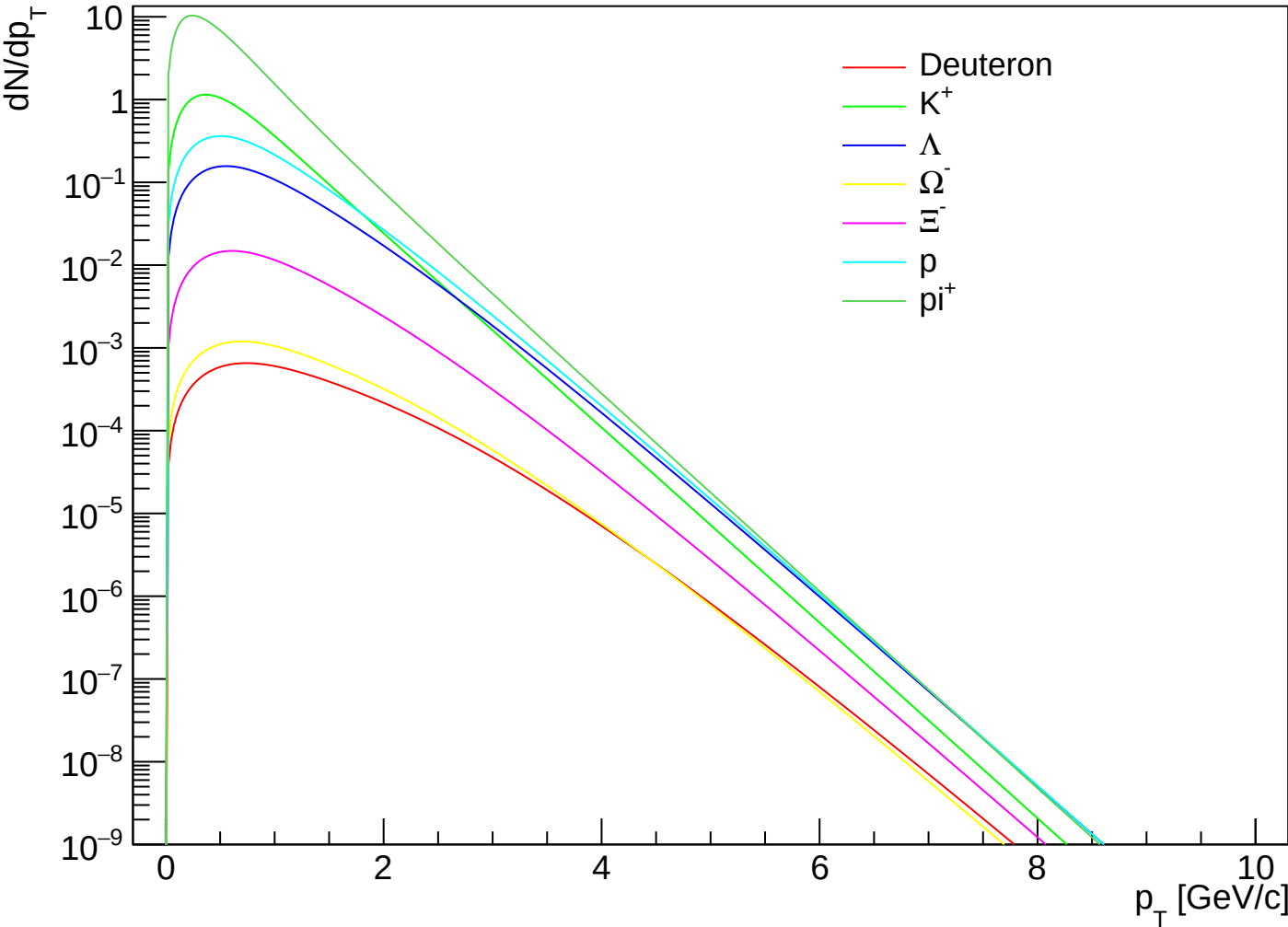
prediction_PbPb5.02_1910.07678_CEGs | k=1.00 | NeNe | cent VIII
