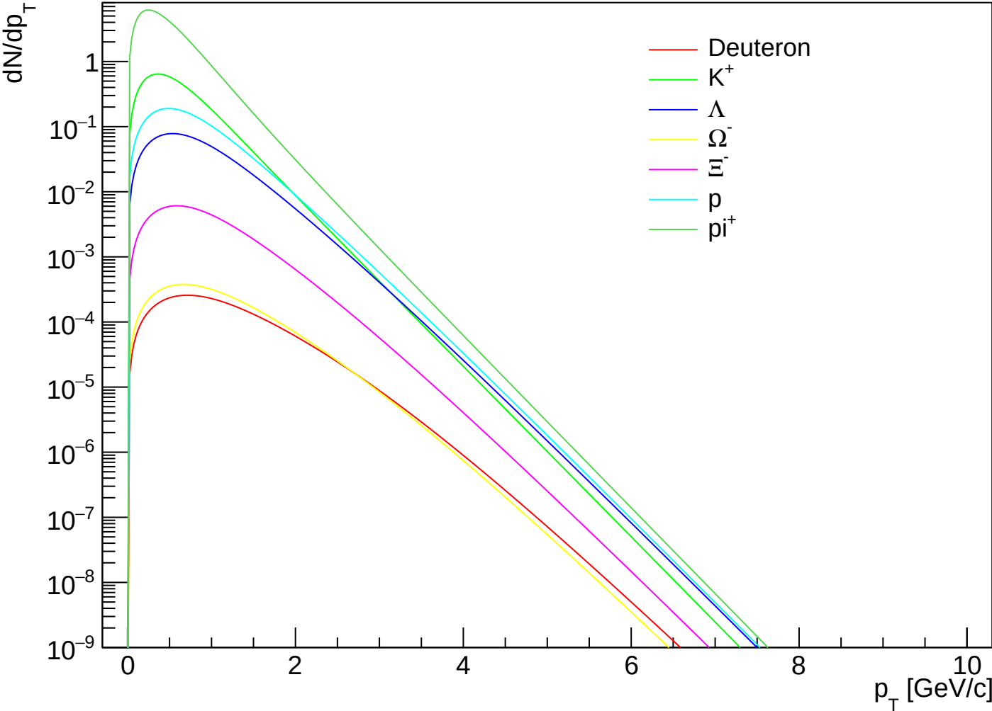
prediction PbPb5.02 1910.07678 CEGs | k=1.00 | pO | cent VII
