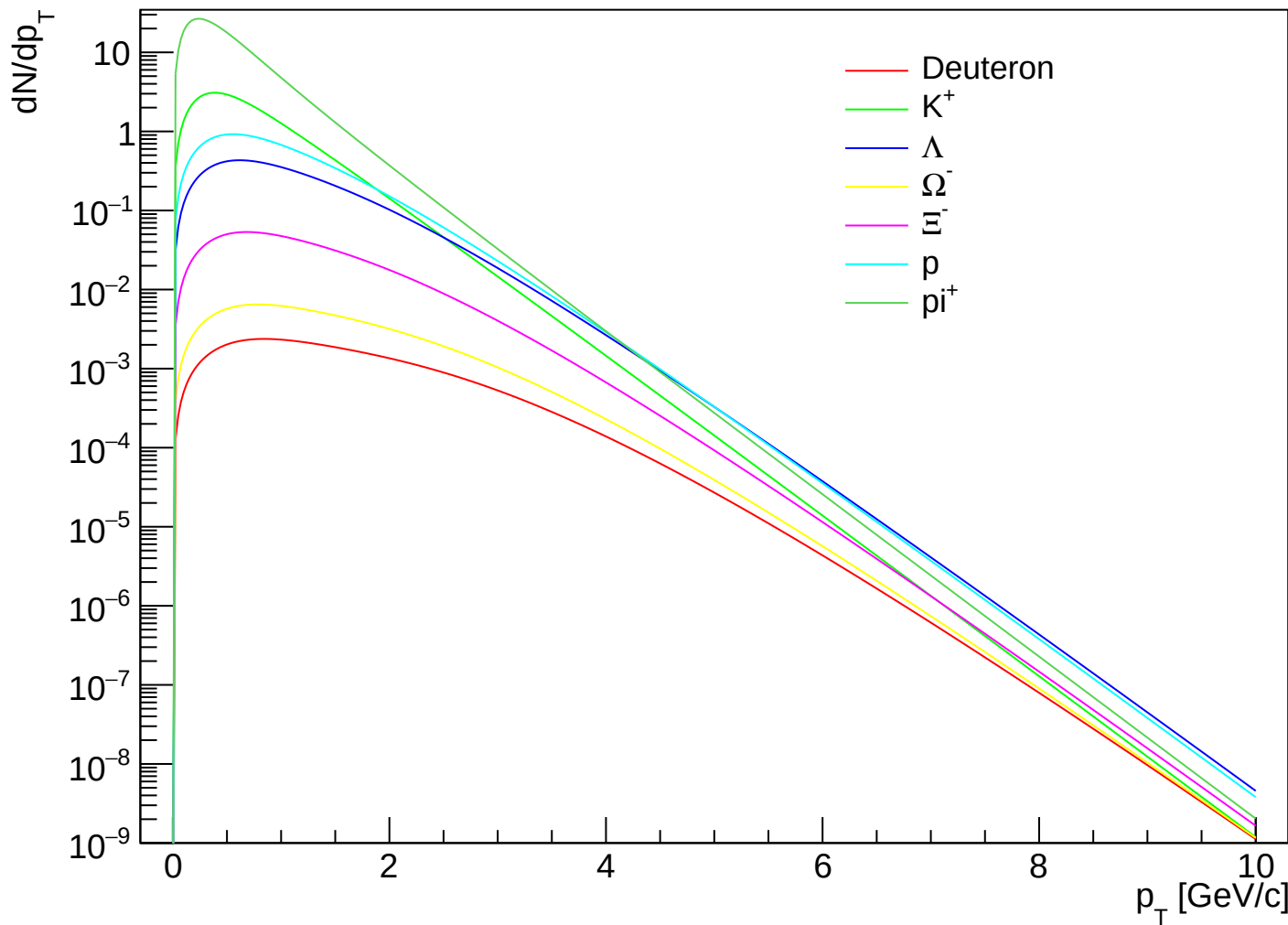
prediction_PbPb5.02_1910.07678_CEGs | k=1.60 | OO | cent VI
