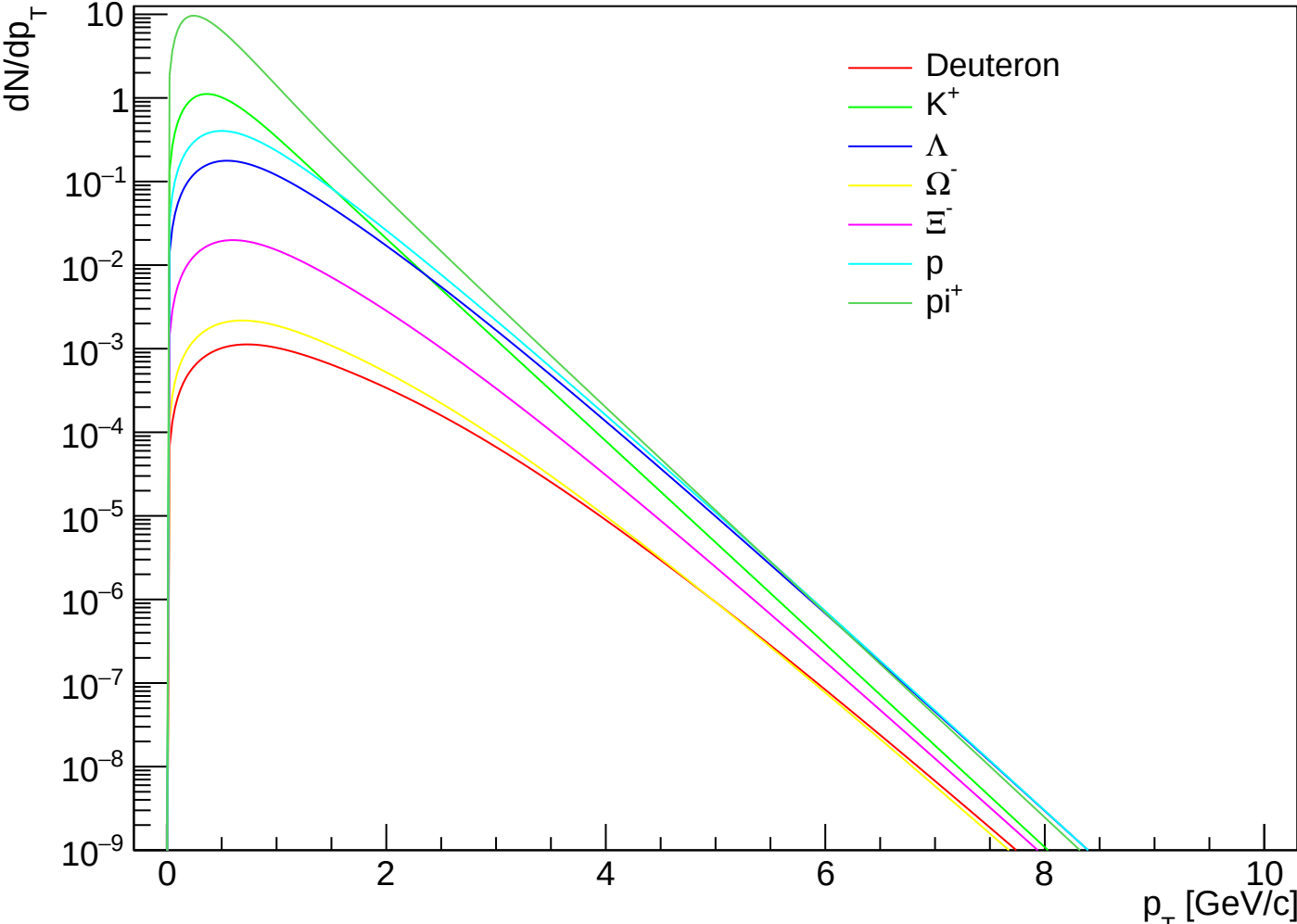
prediction_PbPb5.02_1910.07678_CEGs | k=3.00 | OO | cent VIII
