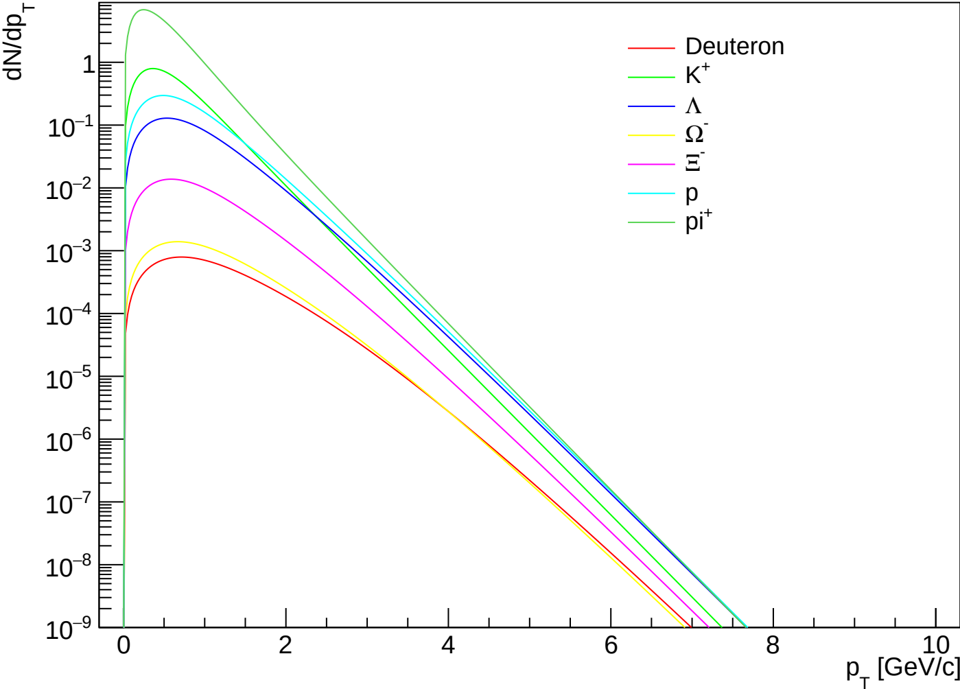
prediction PbPb5.02 1910.07678 CEGs | k=3.00 | pO | cent VII
