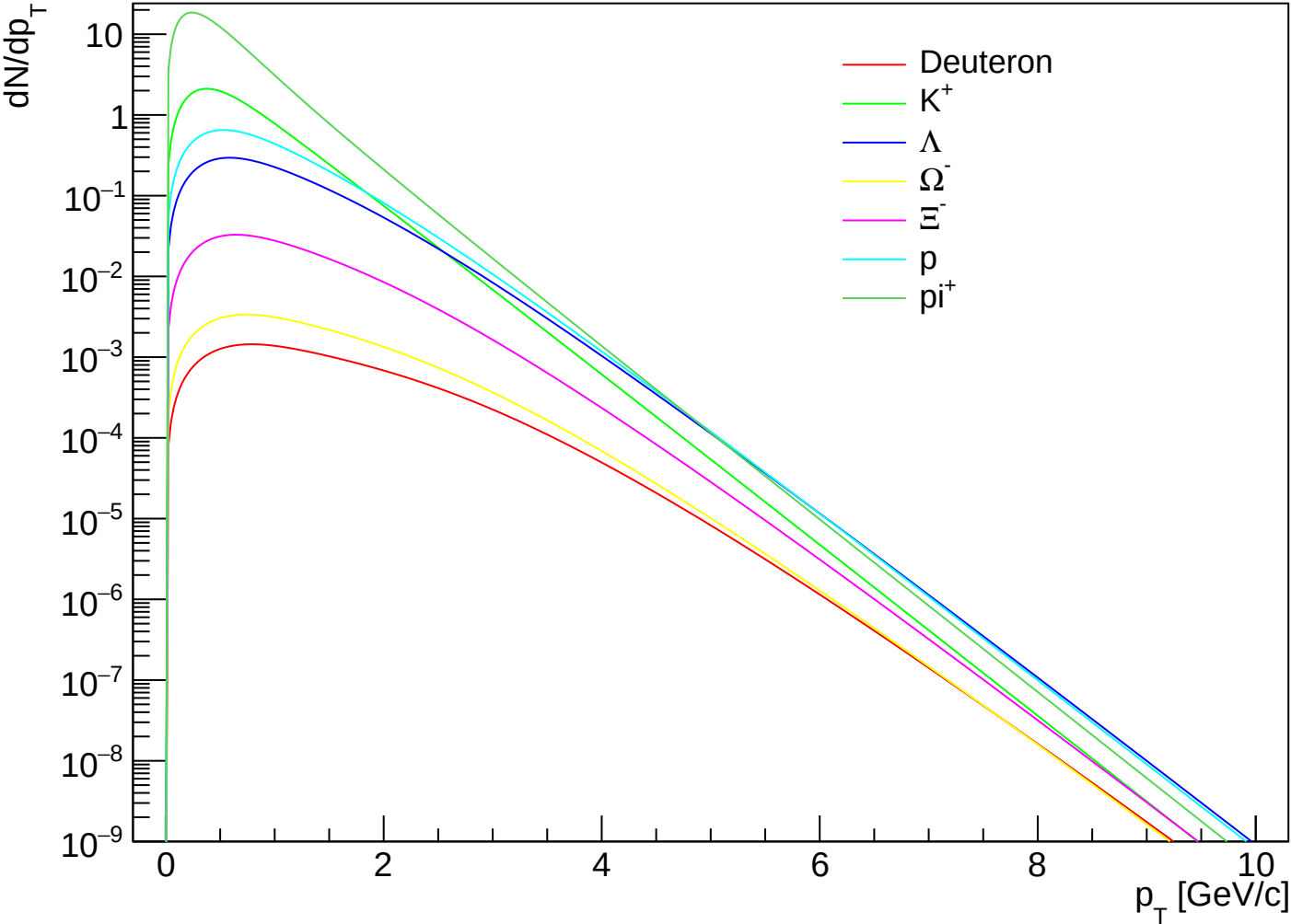
prediction_PbPb5.02_1910.07678_CEGs | k=1.00 | pO | cent II
