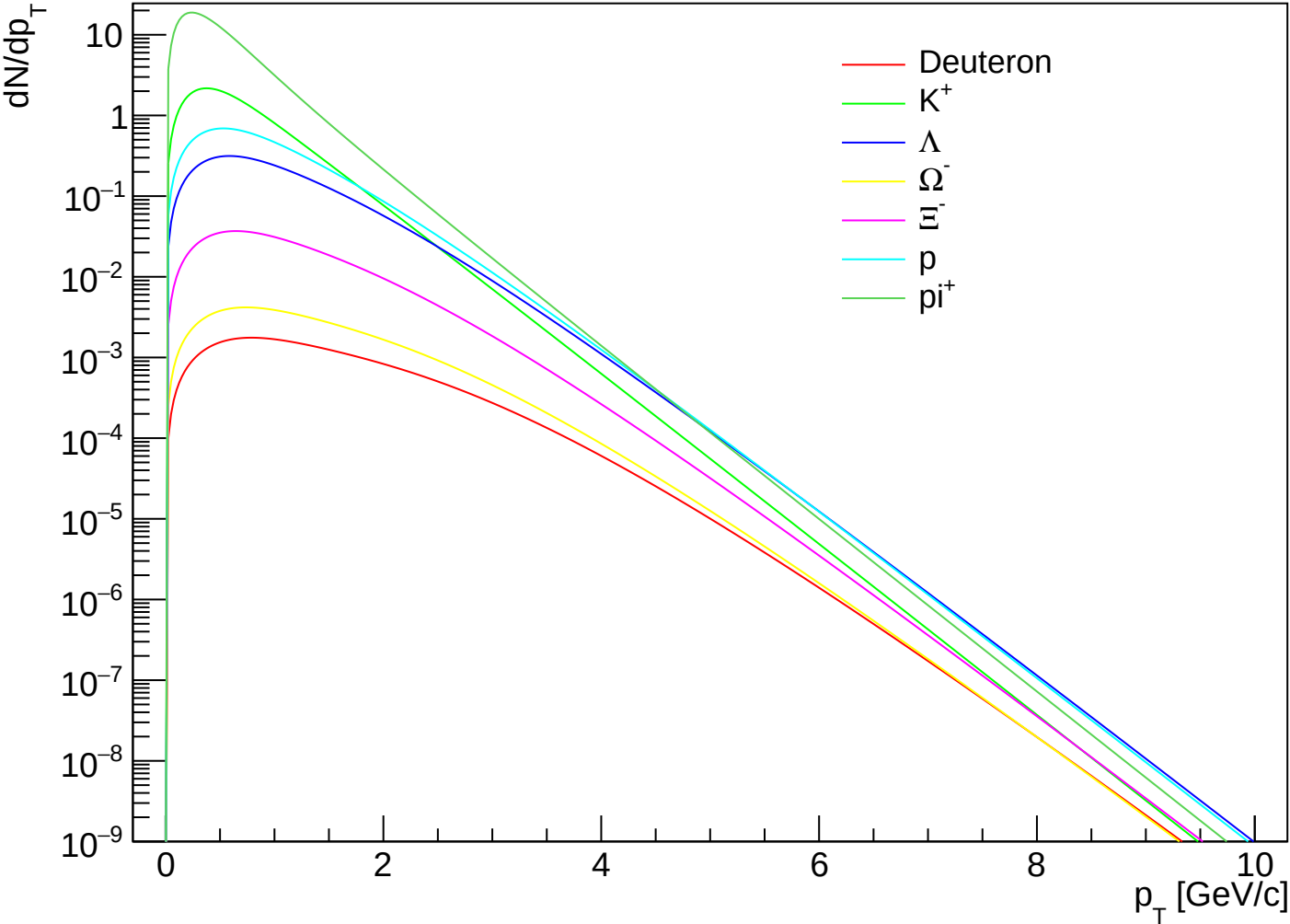
prediction_PbPb5.02_1910.07678_CEGs | k=1.60 | pO | cent II
