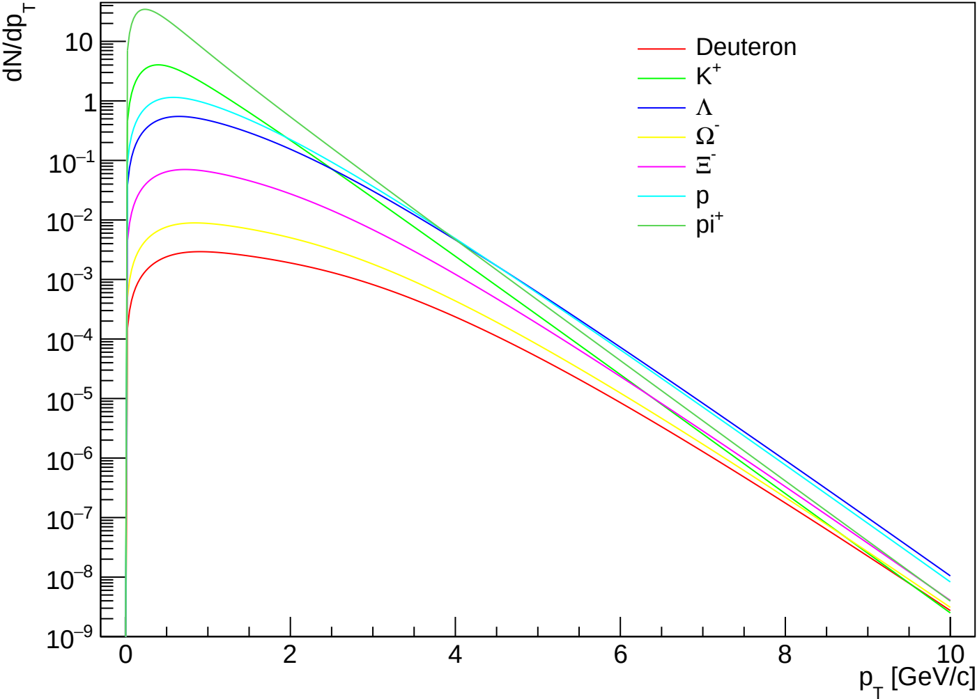
prediction_PbPb5.02_1910.07678_CEGs | k=1.60 | OO | cent V
