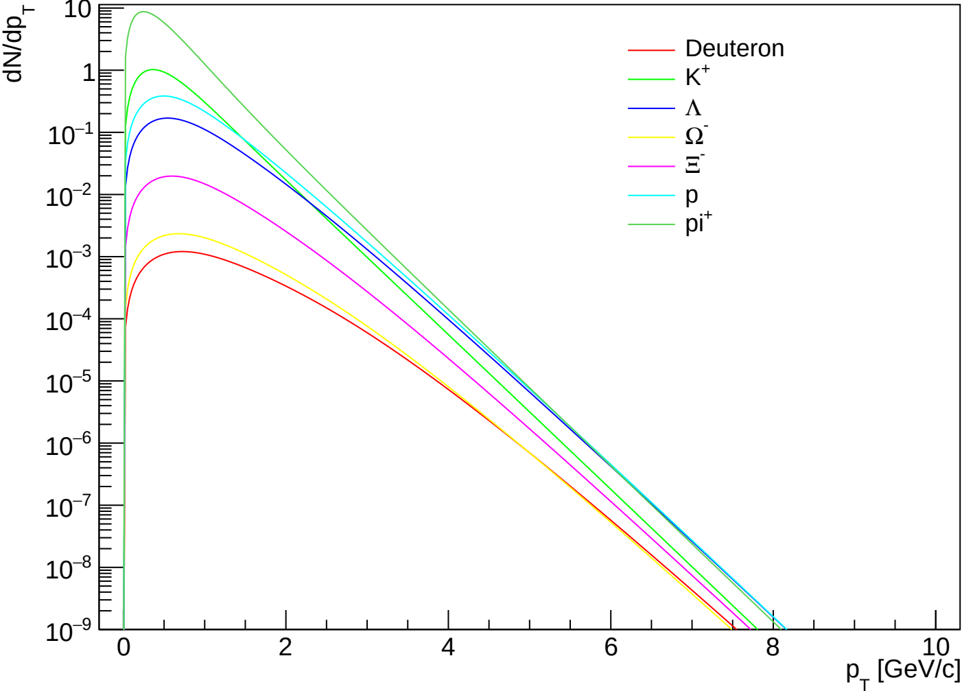
prediction_PbPb5.02_1910.07678_CEGs | k=6.00 | pO | cent VI
