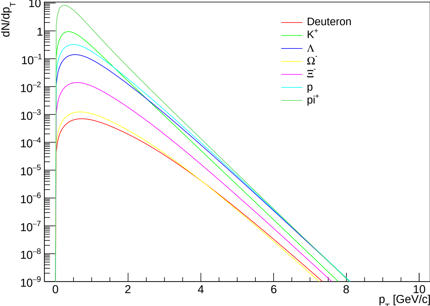
prediction_PbPb5.02_1910.07678_CEGs | k=1.60 | pO | cent VI
