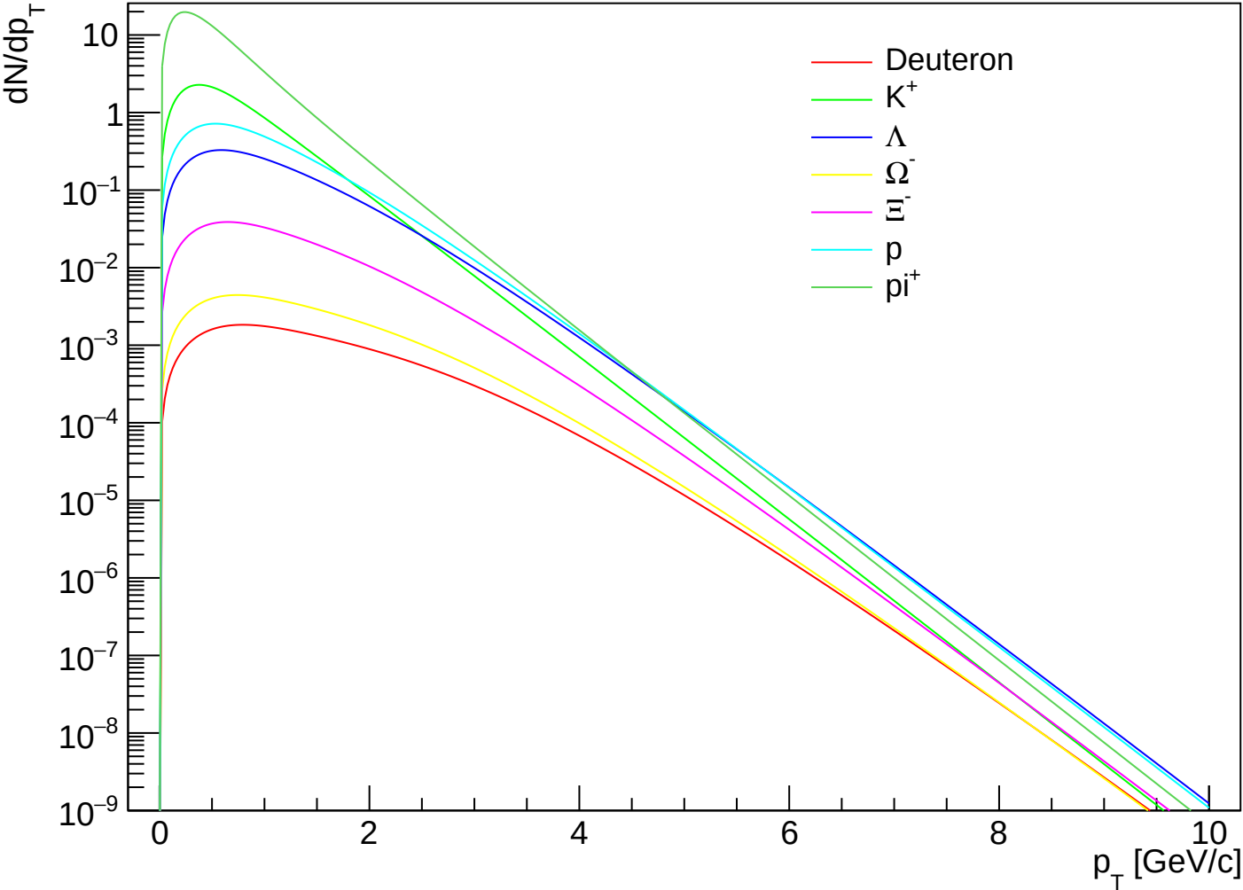
prediction PbPb5.02 1910.07678 CEgs | k=1.60 | OO | cent VII
