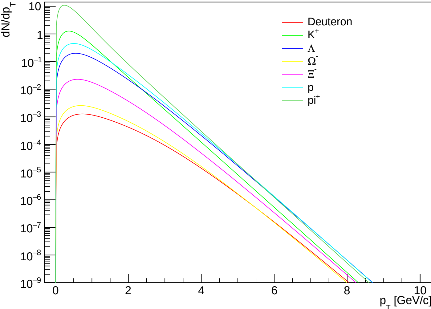
prediction_PbPb5.02_1910.07678_CEGs | k=3.00 | NeNe | cent VIII
