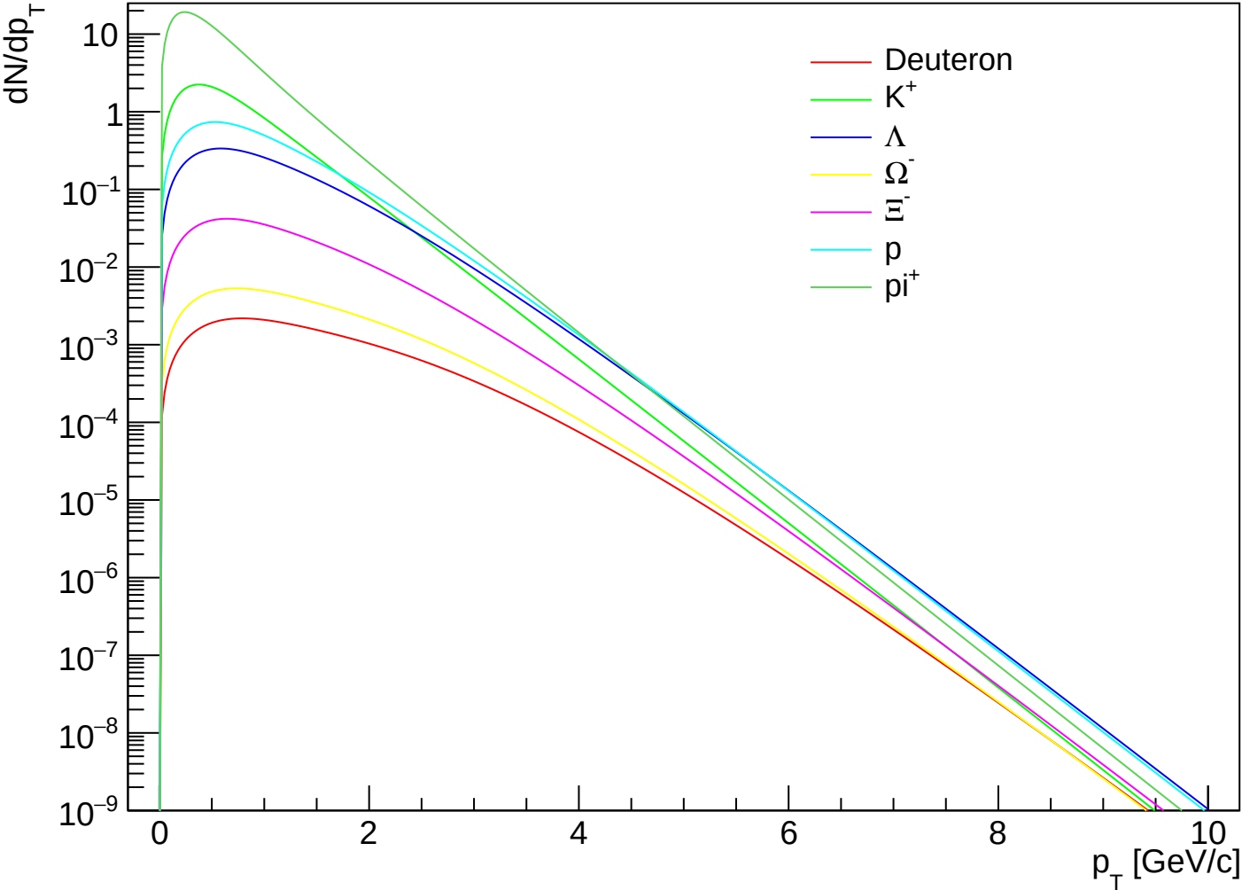
prediction_PbPb5.02_1910.07678_CEGs | k=6.00 | pO | cent II
