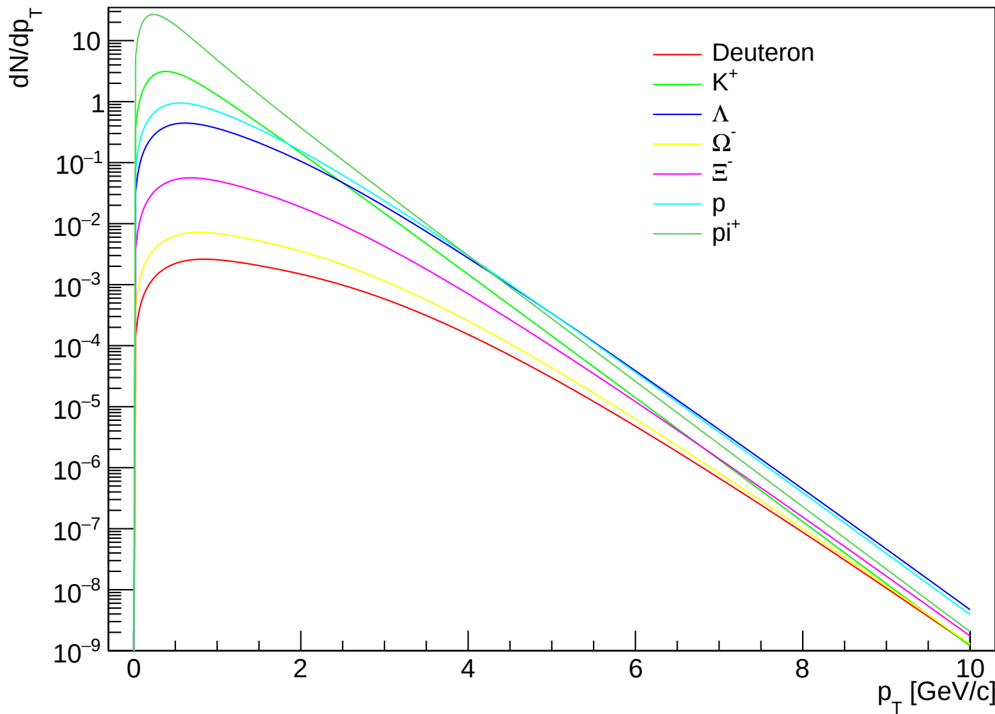
prediction_PbPb5.02_1910.07678_CEGs | k=3.00 | OO | cent VI
