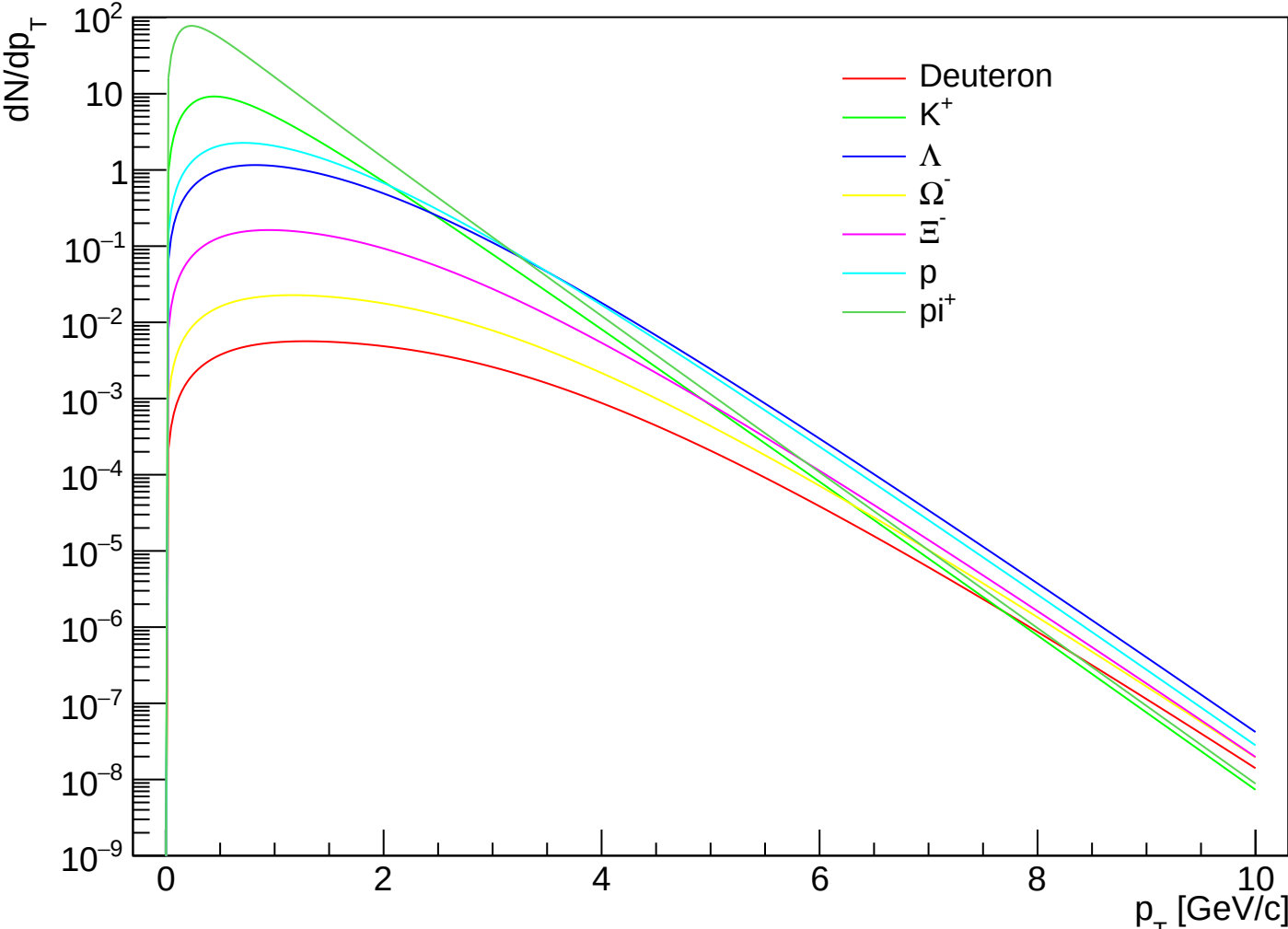
prediction_PbPb5.02_1910.07678_CEGs | k=1.60 | OO | cent I
