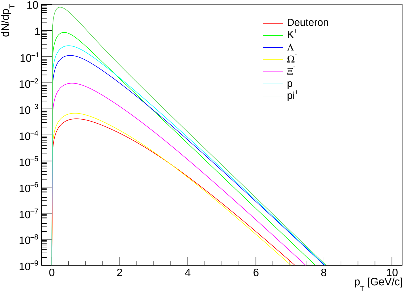
prediction_PbPb5.02_1910.07678_CEGs | k=1.00 | pO | cent VI
