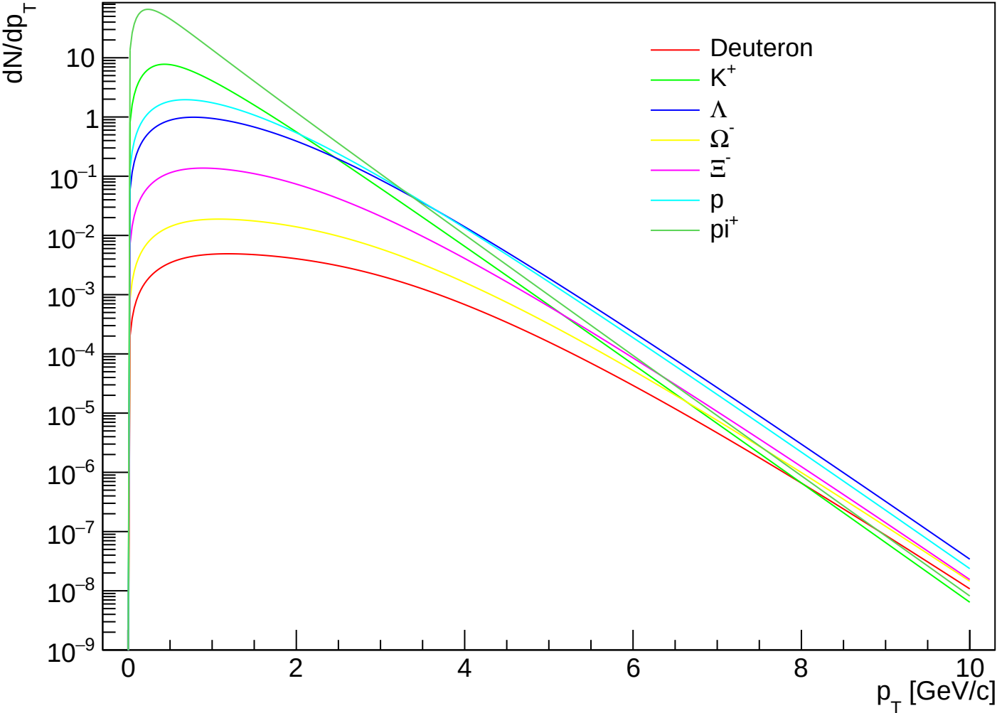
prediction PbPb5.02 1910.07678 CEGs | k=1.60 | OO | cent II
