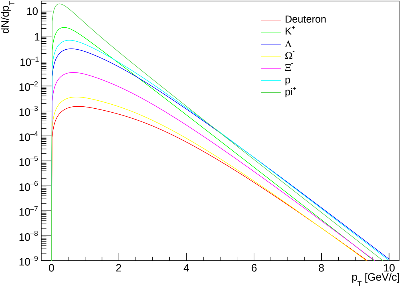
prediction_PbPb5.02_1910.07678_CEGs | k=1.00 | OO | cent VII
