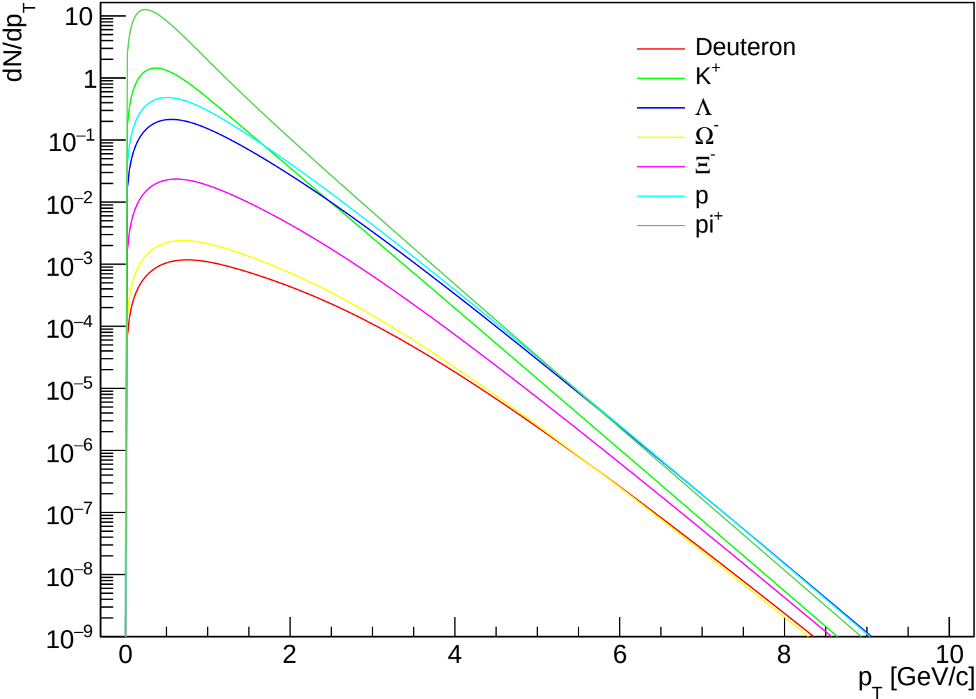
prediction_PbPb5.02_1910.07678_CEGs | k=1.60 | pO | cent IV
