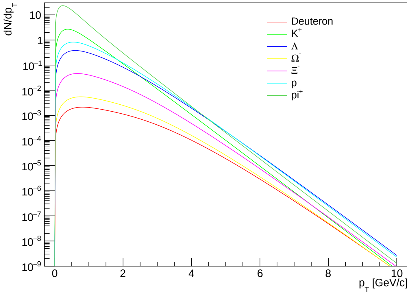
prediction_PbPb5.02_1910.07678_CEGs | k=1.60 | NeNe | cent VII
