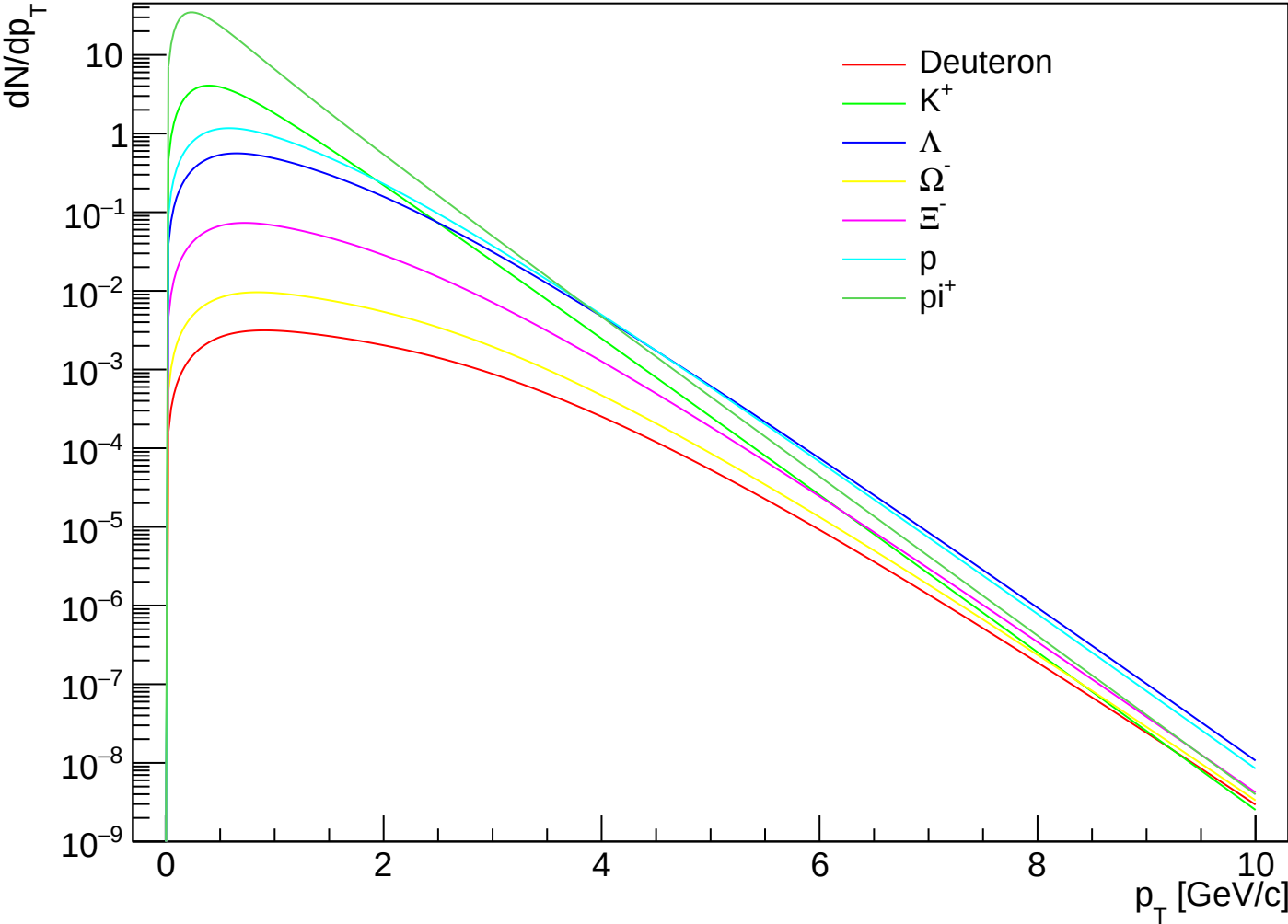
prediction_PbPb5.02_1910.07678_CEGs | k=3.00 | OO | cent V
