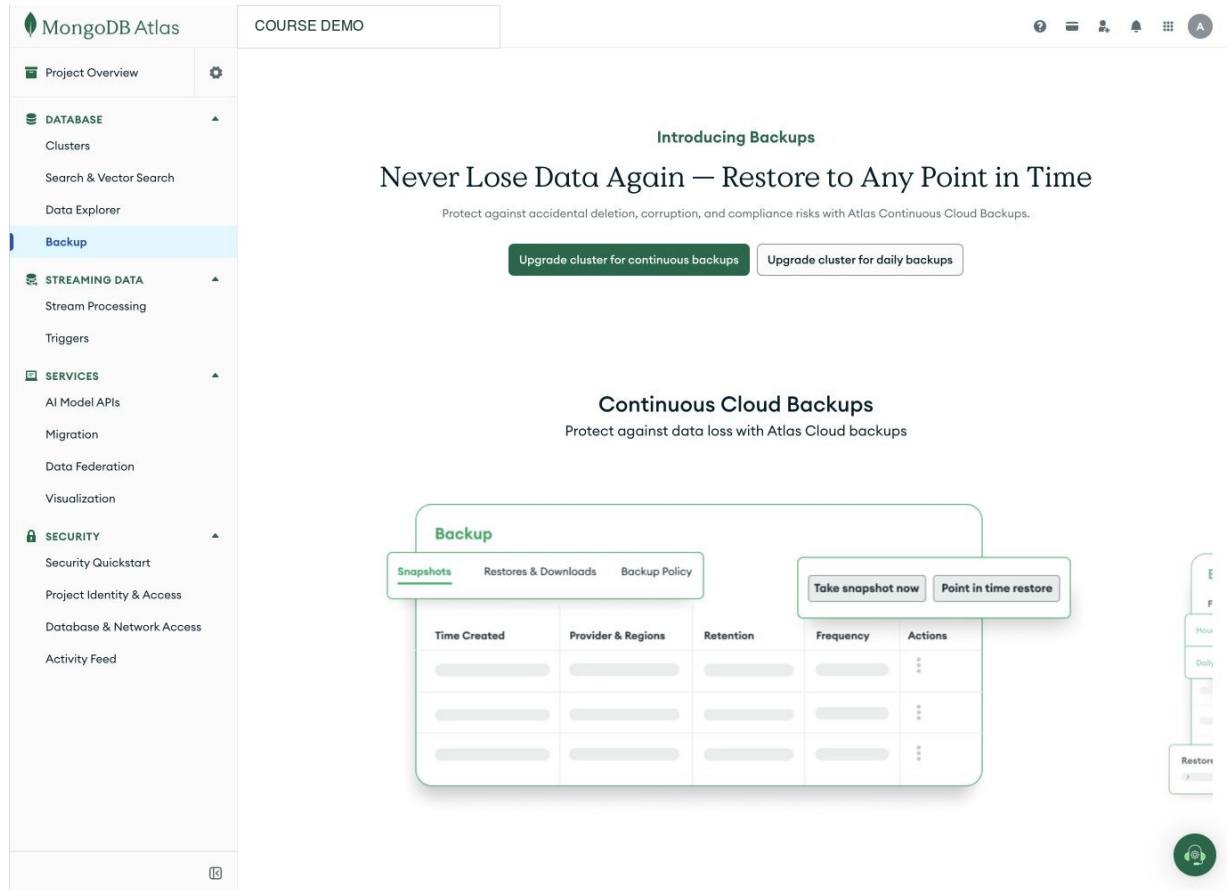
Figure 12.2: The Atlas Free backup screen presents paid continuous or daily backup upgrades rather than an active native backup. A free deployment therefore needs a separate logical recovery plan. Account identifiers are redacted. Interface captured August 25, 2026.
