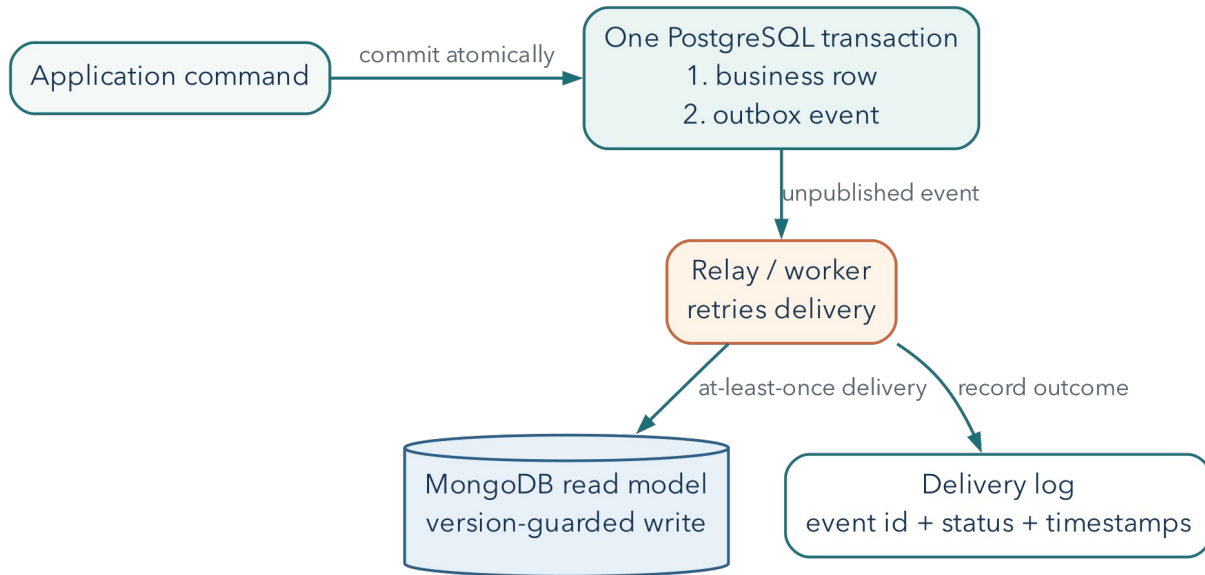
Figure 14.1: A transactional outbox records the business change and event atomically, then delivers an idempotent projection asynchronously.
