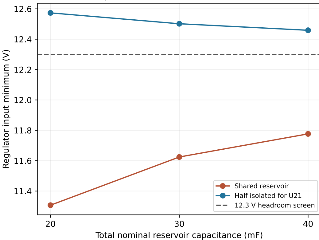
Unbuilt U21 input-isolation candidate — source-only SPICE 2.5 \Omega lamp load, 10 W regulator input, -20% capacitance; assumed transformer and ESR Input minimum at 90% line, 60 Hz
