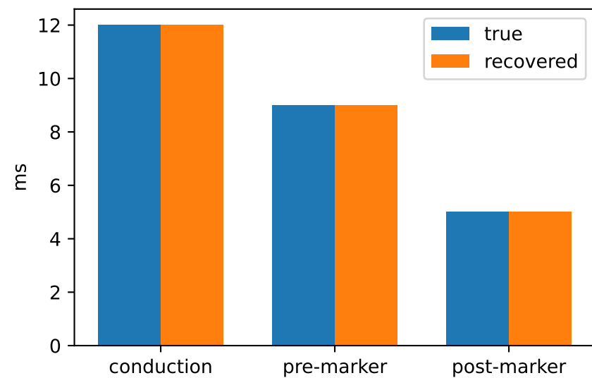
C. Marker differences
