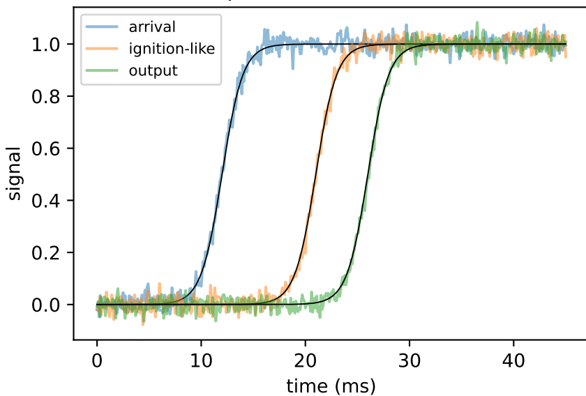
C. Marker differences
