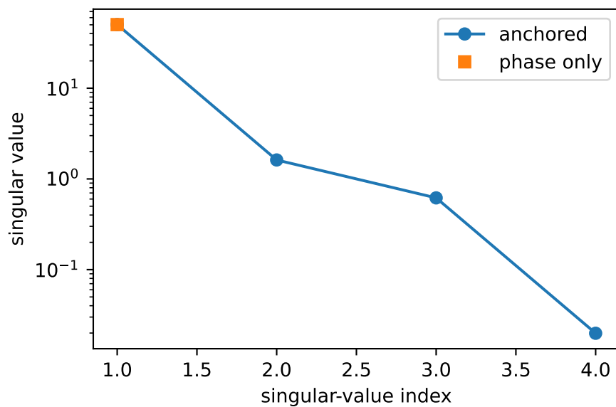
D. Observation ranks: 4 vs 1
