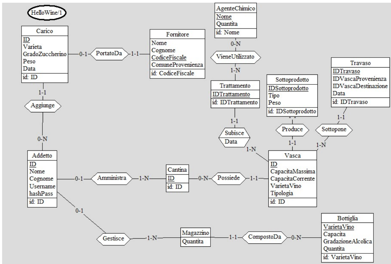
Diagramma E-R:
