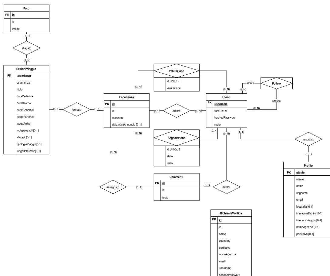
Figura 60: Diagramma logico Entity Relationship
