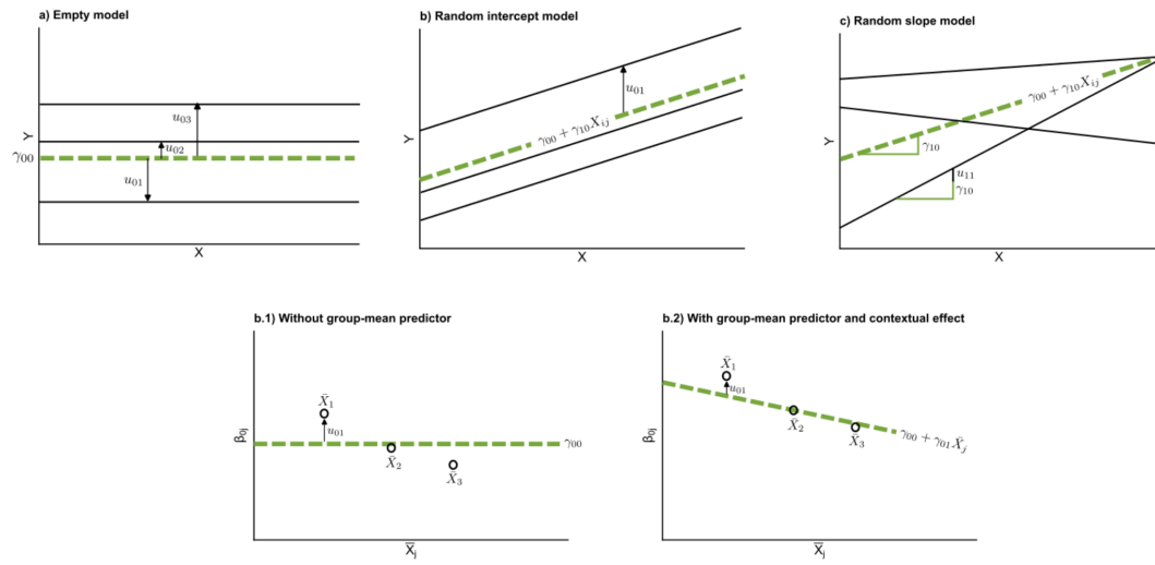
Illustration of common multilevel model specifications. Top row: empty model, random intercept model, and random slope model. Bottom row: group-level relationships between group means of the predictor \bar{X}_{.j} and the group-specific intercepts \beta_{0j} .
