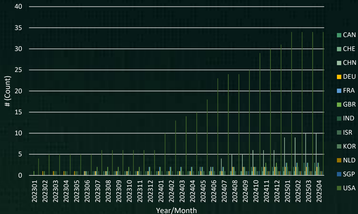
OECD.AI: Number of Model Providers by Country (Oct-2025)
