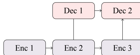
Figure 12.5: Encoder–decoder Transformer schematic with cross-attention.
