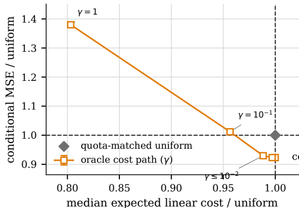
(a) MSE--cost frontier
