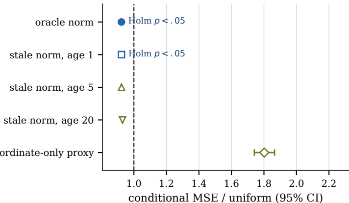
(b) Oracle and proxy policies
