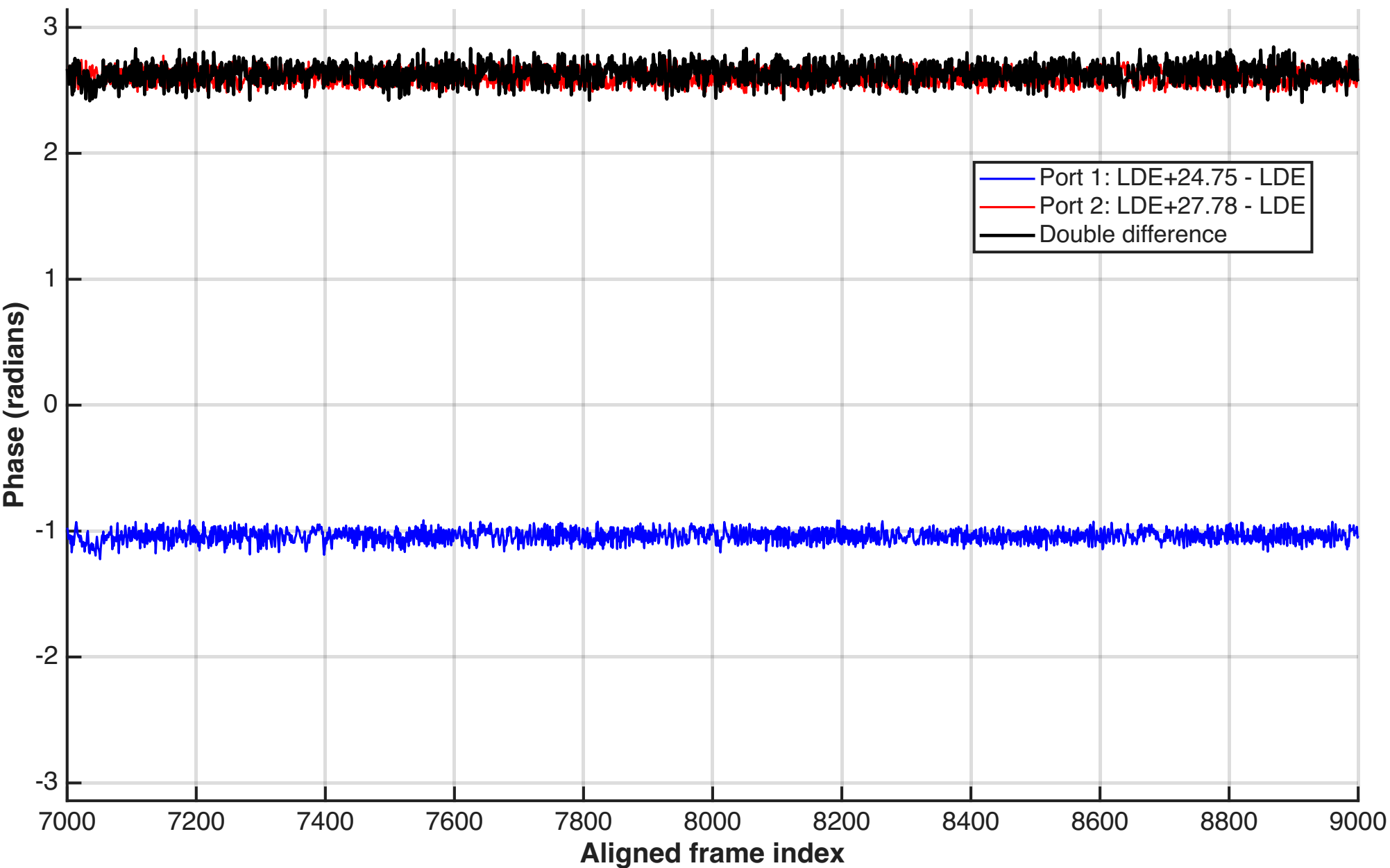
Cable Phase Fluctuation Referenced to LDE
