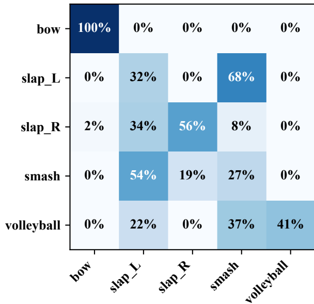
Predicted label
