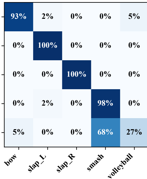
Predicted label
