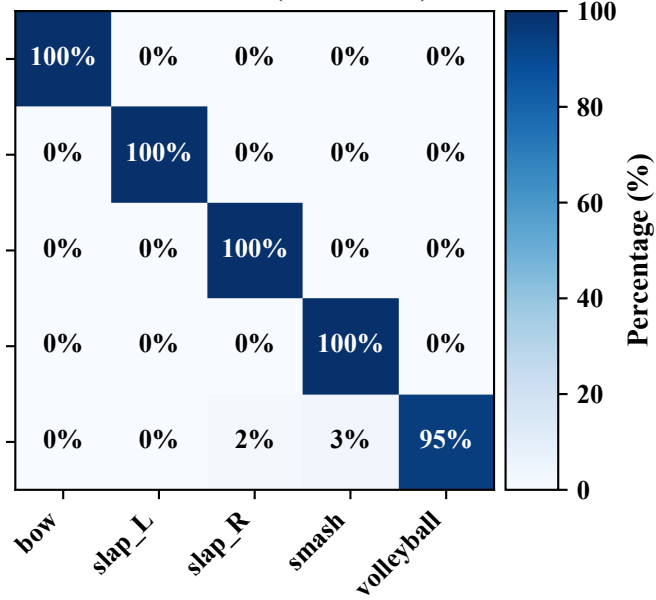
Predicted label
