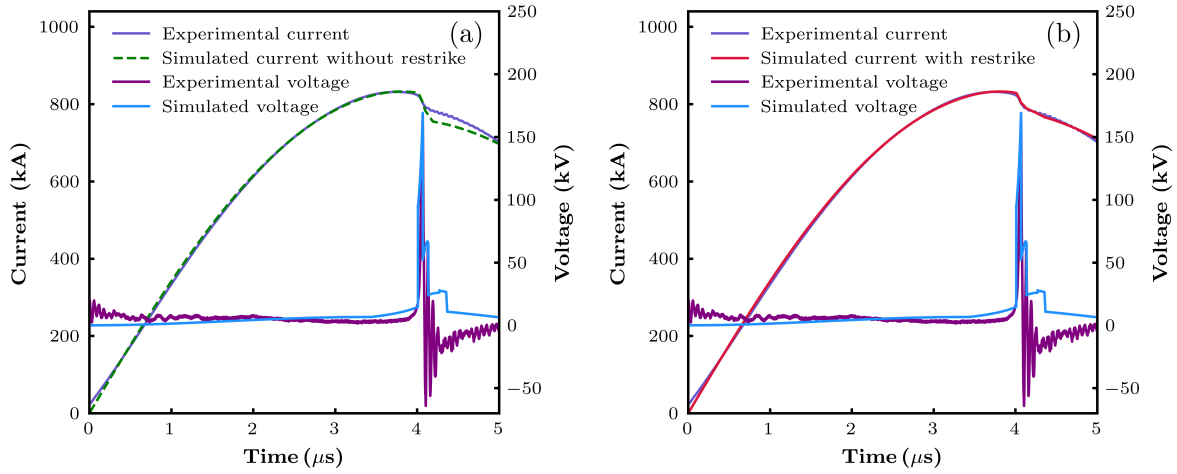
Figure 2. (a) Showing the inability of fitting the current dip with one set of radial model parameters. (b) Showing good fitting of the current dip using a second set of radial model parameters at the transition (re-strike) time. Note that the transition time correlates to the time of peak voltage.
