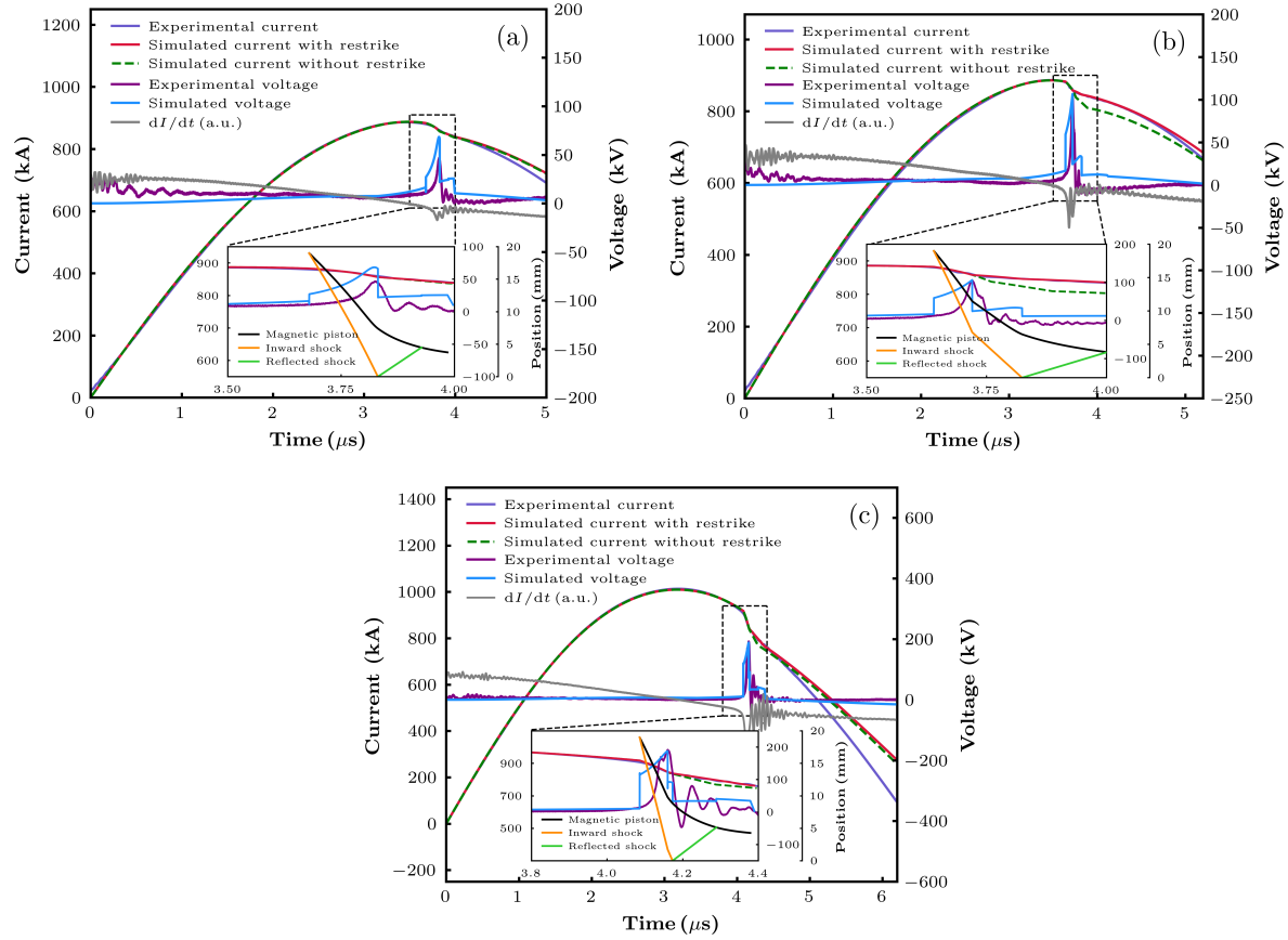
Figure 5. Comparing current, voltage, and dynamics of 3 shots across the range of yields and voltage spikes. (a) Shot 1062 at 100 kV with D-D mixture at 12 Torr, showing a low yield shot, (b) Shot 1036 at 100 kV with D-D mixture at 12 Torr, showing an average yield shot, and (c) Shot 895 at 100 kV with D-D mixture doped with 0.1 Torr Kr, showing highest f_{cr} and highest V_p .
