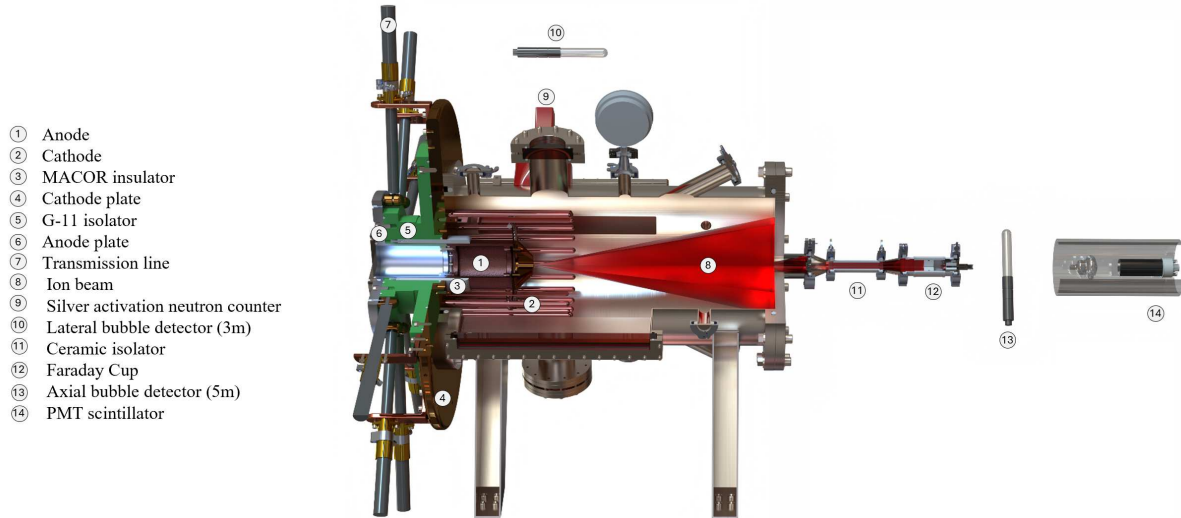
Figure 1. A sectional sketch of F-I with a schematic of the ion beam emitting in a cone and an ion sample being measured by the Faraday Cup. The collector plates are illustrated on the left with several coaxial cables from the capacitor bank. The tapered anode and circle-of-rods cathode are also presented. Positions of two bubble detectors and a photomultiplier-scintillator are shown.
