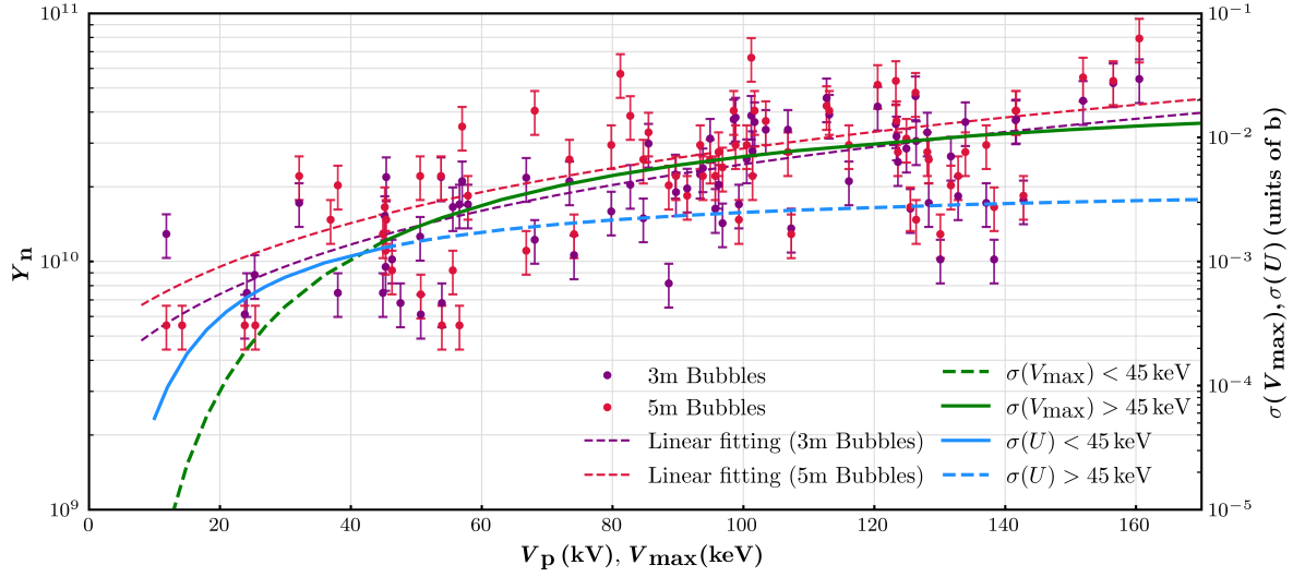
Figure 3. Correlation of measured neutron yield versus peak voltage V_p also designated as V_{\max} with D-D beam-target fusion cross section \sigma(V_{\max}) versus V_{\max} and \sigma(U) vs. V_{\max} , where U = 3V_{\max} is the effective inductive voltage used in the Lee code.
