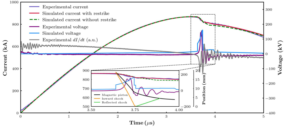
Figure 4. The fitting of current traces is shown in the main chart together with the voltage waveforms. The inset shows the correlation of radial phase dynamics with the fitted current dips and voltage spikes. The position of the shock front and piston at the start of the radial phase at 3.64 \mu\text{s} is 19 mm.
