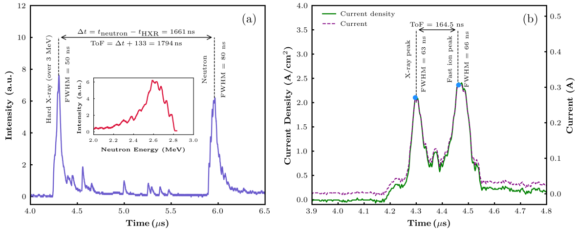
Figure 6. a) Lead-shielded PM-Scintillator signal at 16 Torr with a time-of-flight of 1794 ns and flight length of 40 m. b) FC signal at 16 Torr with a time-of-flight of 164.5 ns.
