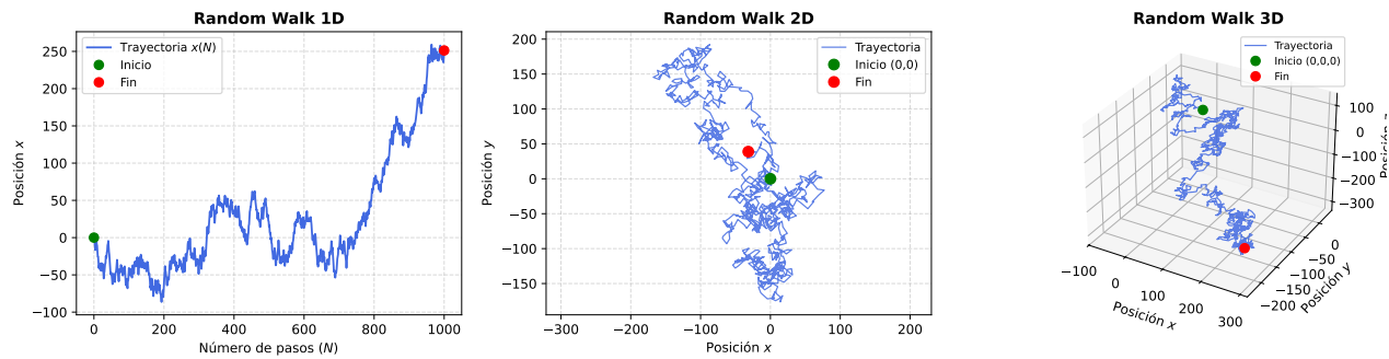
Figura 4: Random walk.
