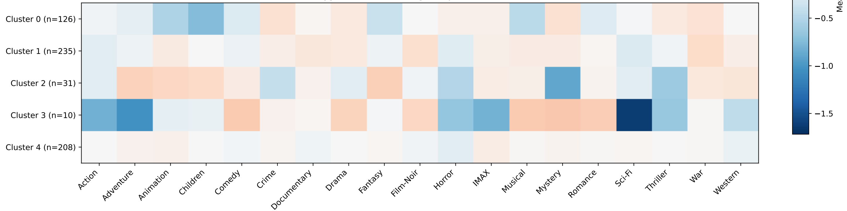
Agglomerative Ward: genre profiles at K = 5
