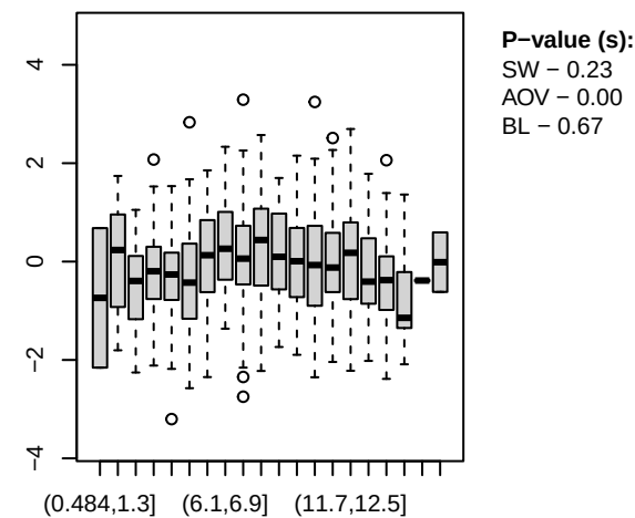
HNB Linear, k = 20
