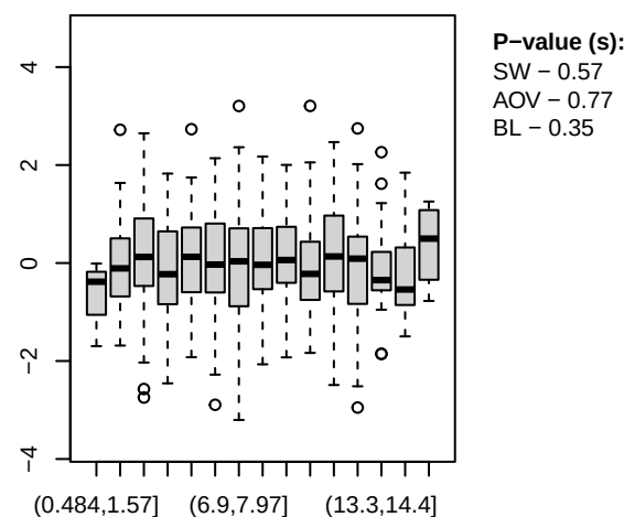
HNB Nonlinear, k = 15
