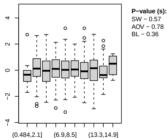
HNB Nonlinear, k = 10
