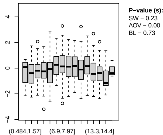
HNB Linear, k = 15
