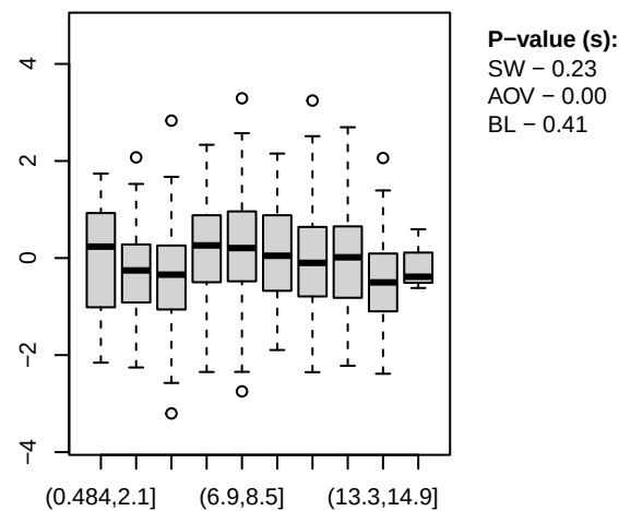
HNB Linear, k = 10
