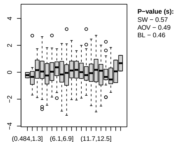
HNB Nonlinear, k = 20
