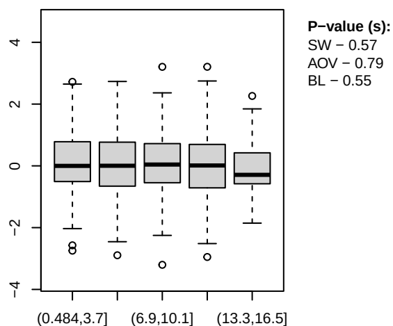
HNB Nonlinear, k = 5
