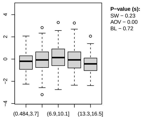
HNB Linear, k = 5
