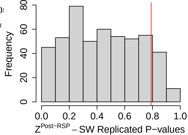
(c) HNB Linear, Z^{\text{Post-RSP}} - SW P-values
