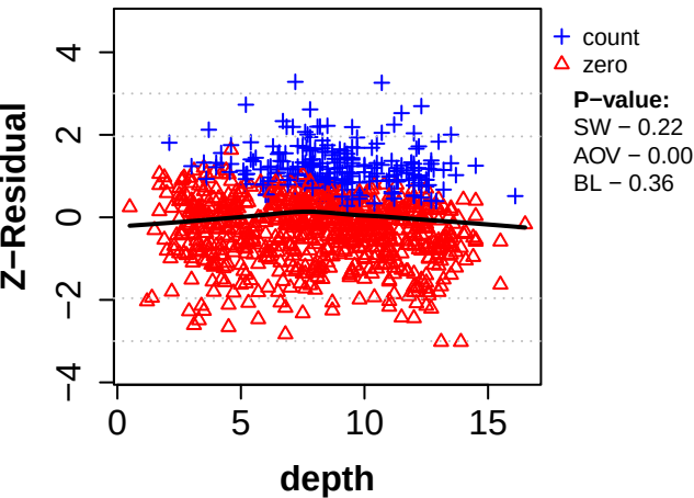
(a) HNB Linear, Z^{\text{Post-RSP}} Scatterplot
