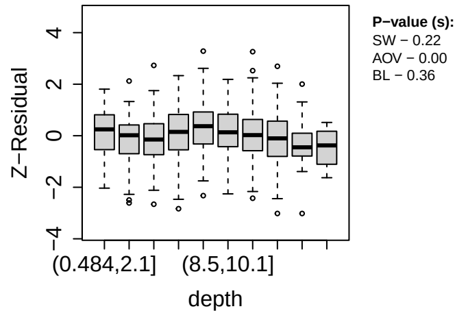
(b) HNB Linear, Z^{\text{Post-RSP}} Boxplot
