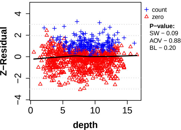
(a) HNB Nonlinear, Z^{\text{Post-RSP}} Scatterplot
