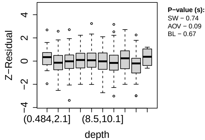
(b) HNB Nonlinear, Z^{\text{Post-RSP}} Boxplot
