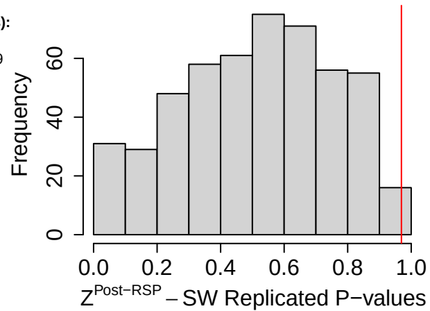
(c) HNB Nonlinear, Z^{\text{Post-RSP}} - SW P-values
