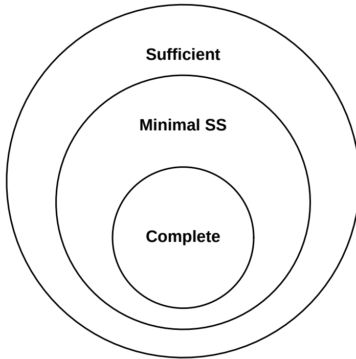
Figure 9.2: Hierarchy of Statistics: Completeness implies Minimal Sufficiency under regularity.
