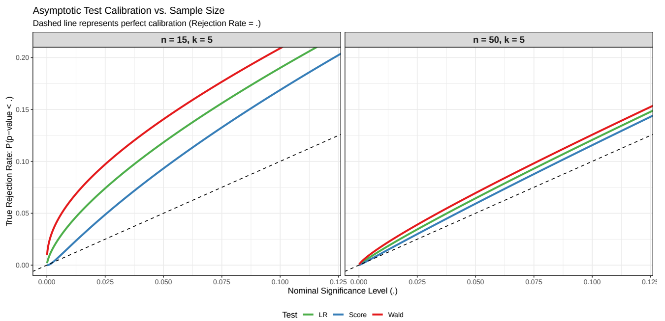
Figure 8.2: Exact Analytical CDFs of Asymptotic P-values
