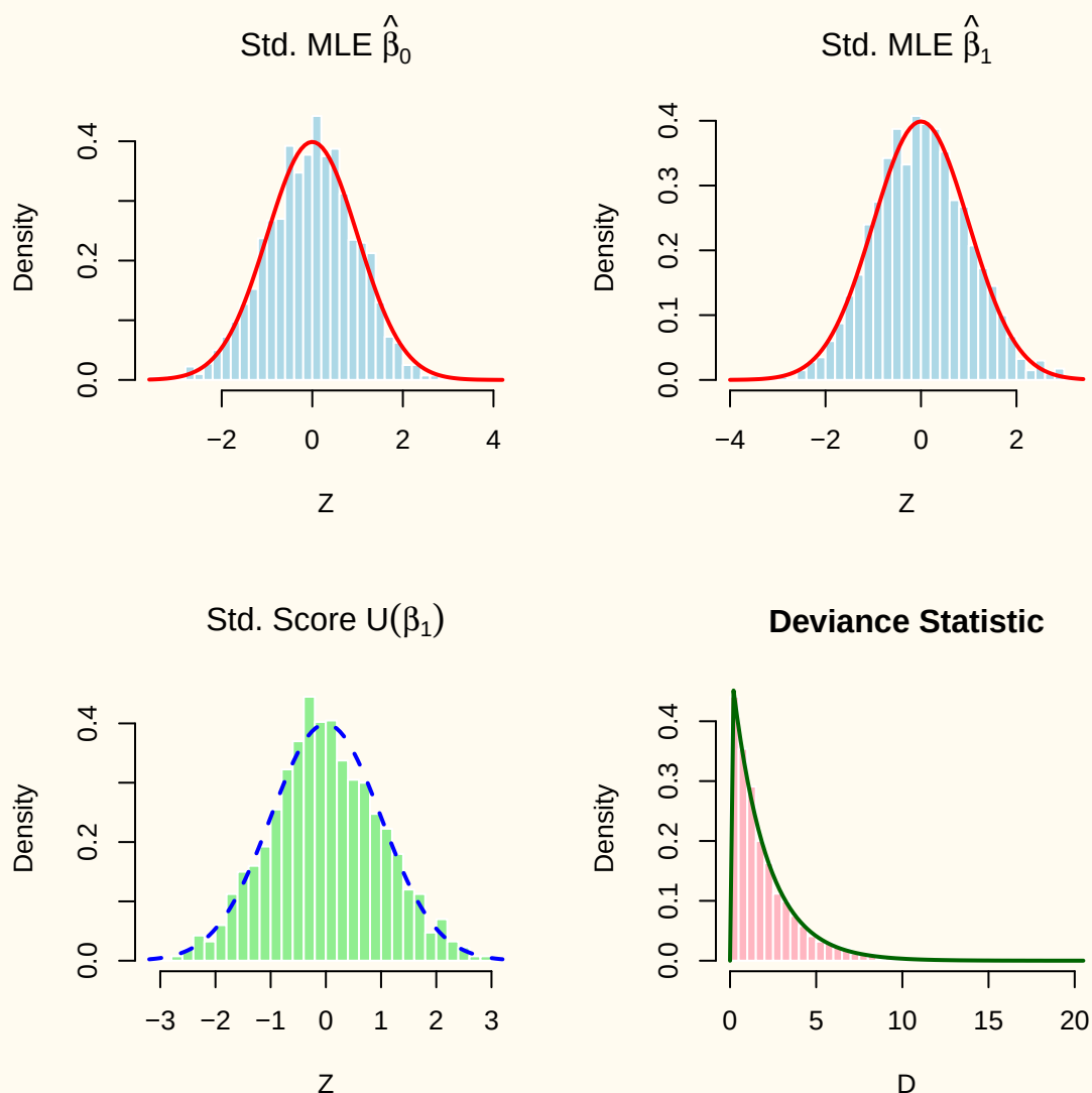
Figure 6.7: Asymptotic distributions for Poisson Regression (n=200). Top Row: Standardized MLEs for Intercept and Slope (Normal). Bottom Left: Standardized Score for Slope (Normal). Bottom Right: Deviance Statistic (Chi-squared with 2 df).
