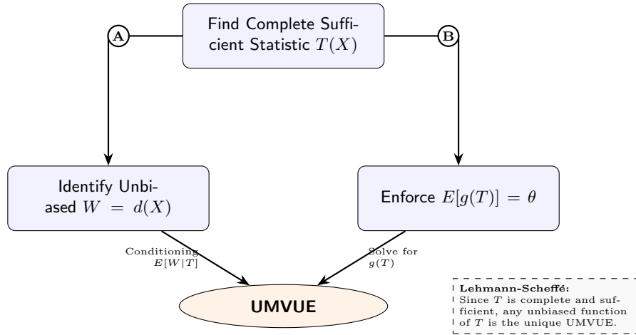
Figure 9.3: The two paths to finding the UMVUE: (A) Rao-Blackwellization via conditioning an initial unbiased estimator W on T ; (B) The Direct Method by solving for an unbiased function g(T) directly.
