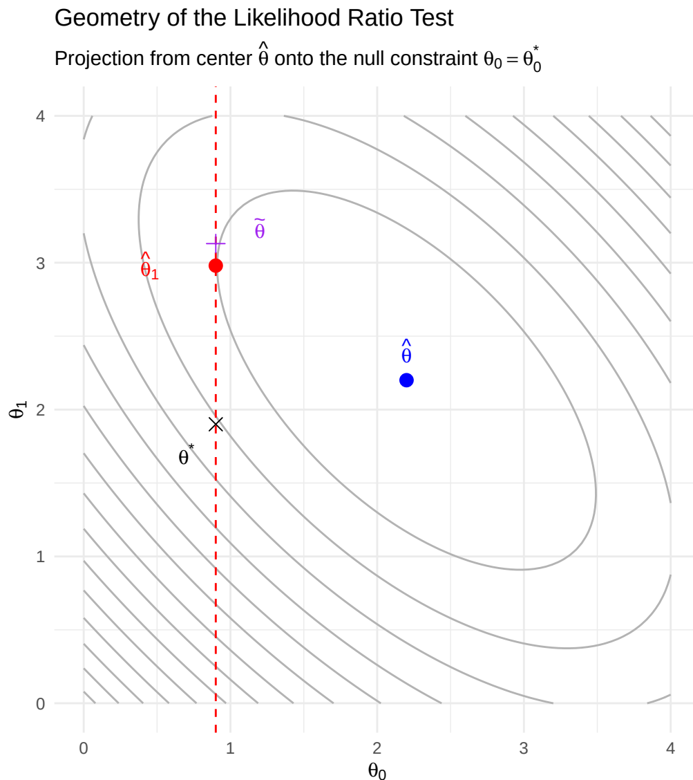
Figure 8.1: The geometry of restricted optimization. Blue dot is the unrestricted MLE (center). The red dot represents the projected nuisance parameter center on the null line. The purple cross is the restricted MLE.
