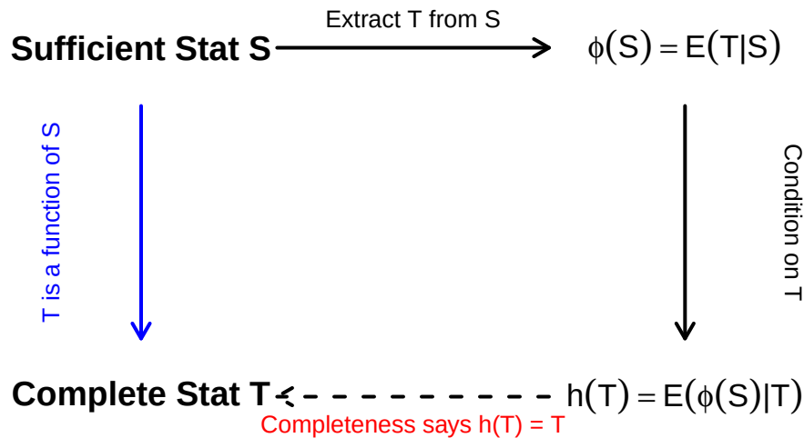
Figure 9.1: Logical flow of the proof: Showing T is a function of any sufficient statistic S .
