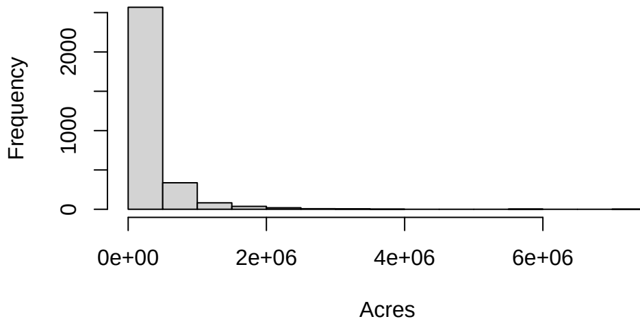
Histogram of 1992 Acres
