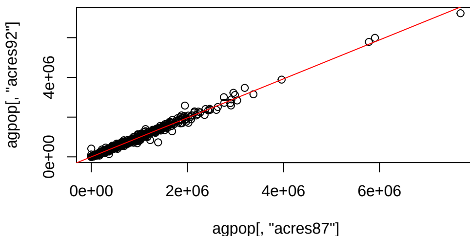
Acres 1992 vs Acres 1987
