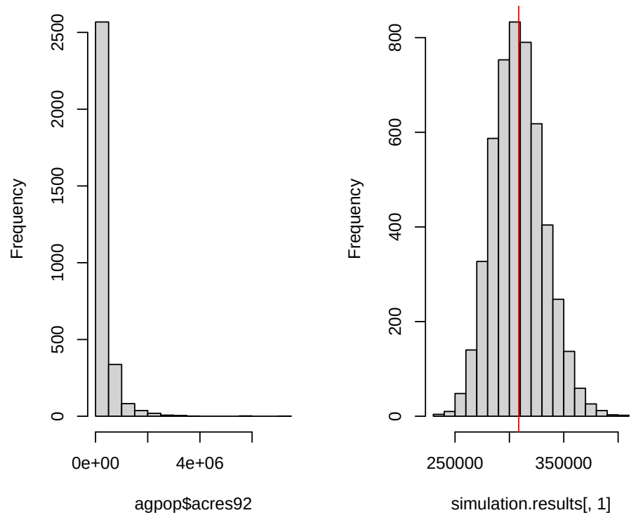
Population Distribution of acre9ling Distribution of Sample Mean f
