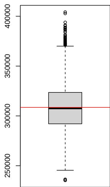
Boxplot of Sample Mean
