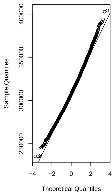
QQ plot of Sample Mean
