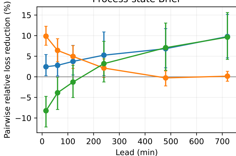
Process-state Brier
