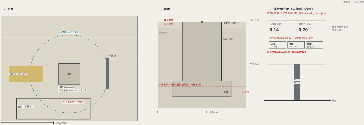
FIG.16 The benchmark and its reading plate, as a construction detail
