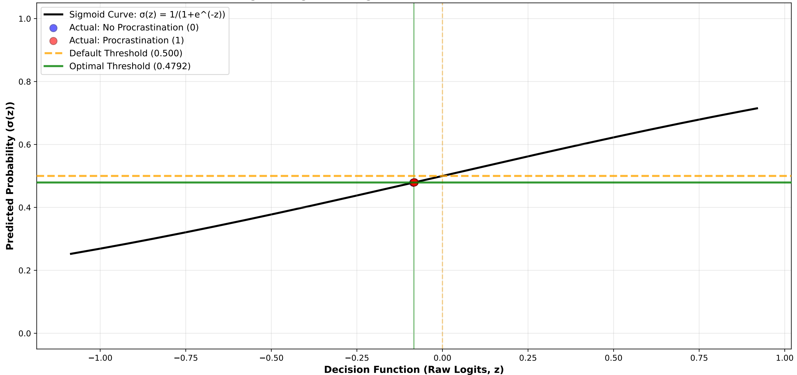
Logistic Regression Sigmoid Curve with Decision Boundaries
