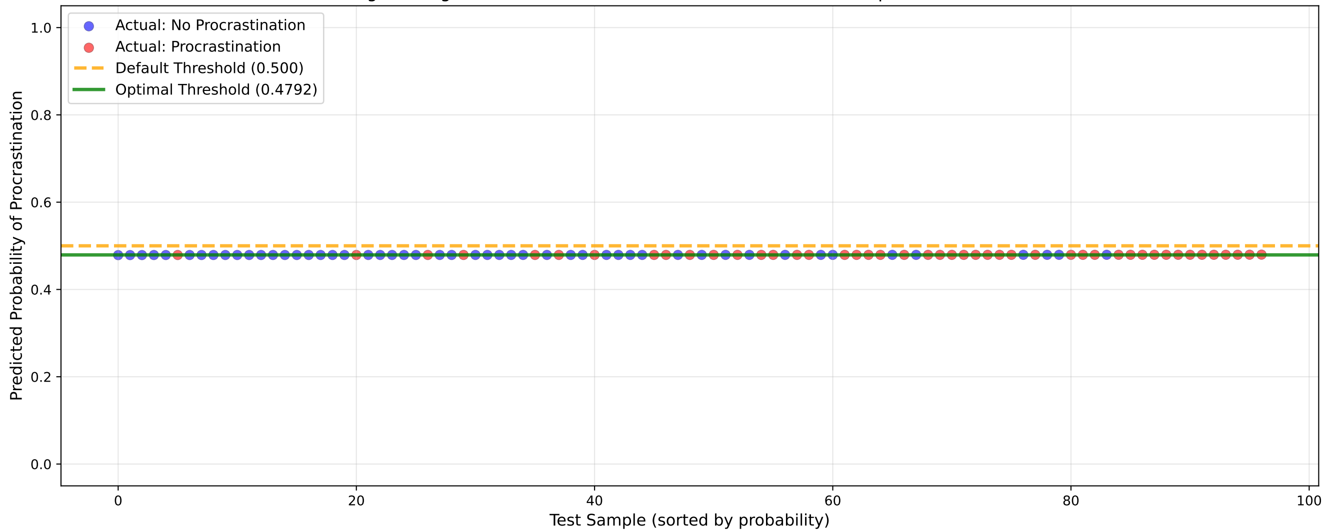
Logistic Regression: Predicted Probabilities with Default vs. Optimal Thresholds
