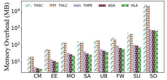
Figure 8: Memory overhead (excluding the graph itself).
