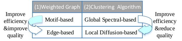
Figure 3: Key functions of the seminal two-stage framework.
