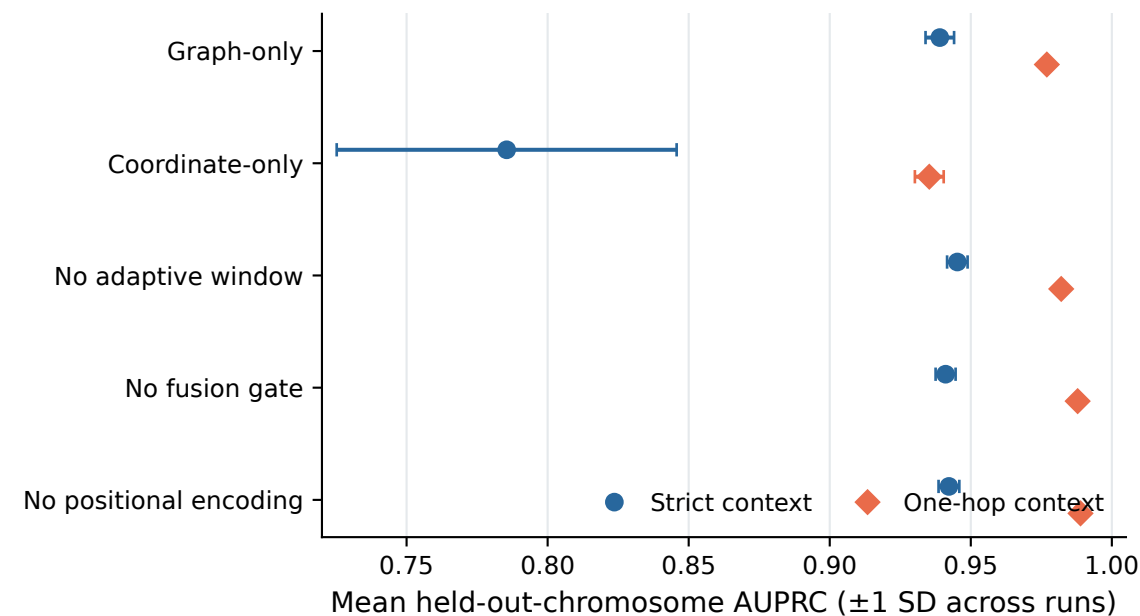
c Model-component controls
