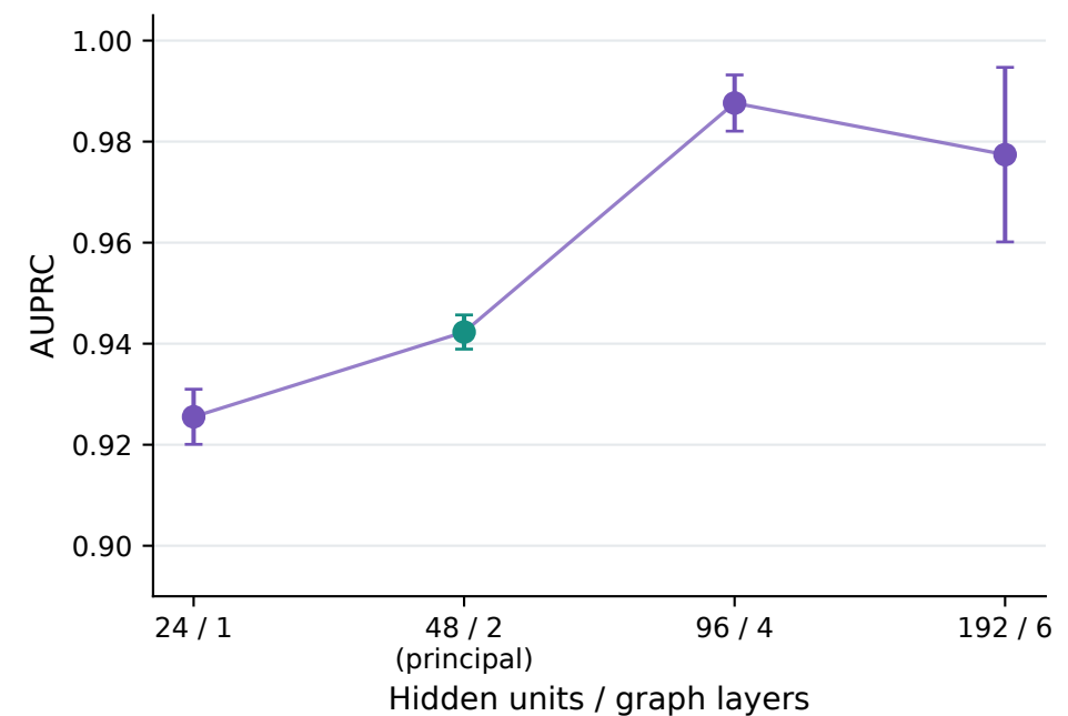
d Capacity sweep under strict context
