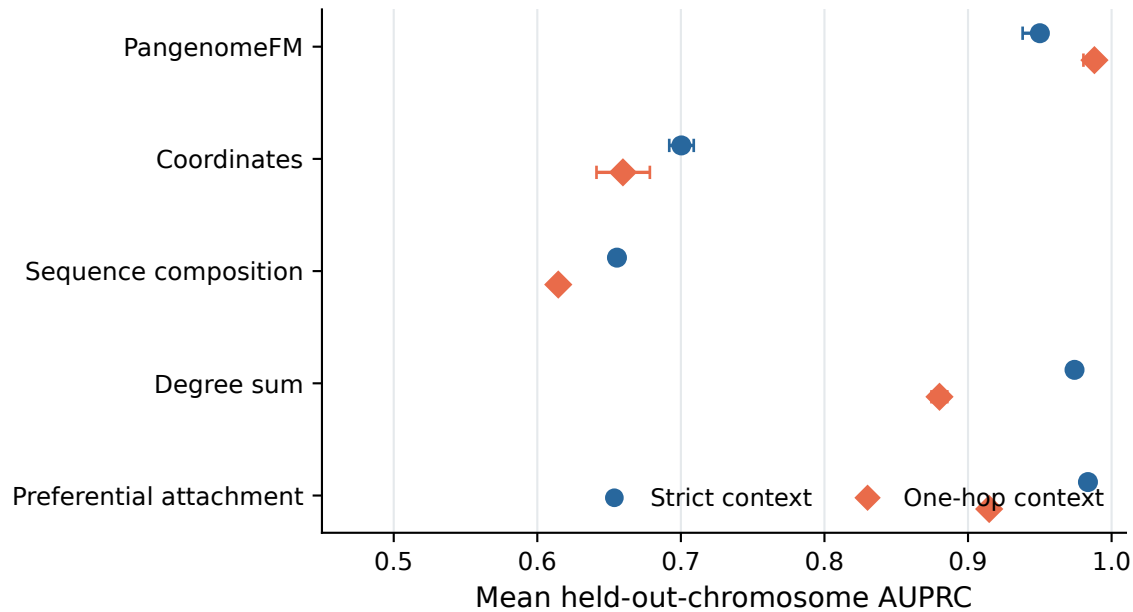
a Hidden-connection reconstruction versus simple baselines
