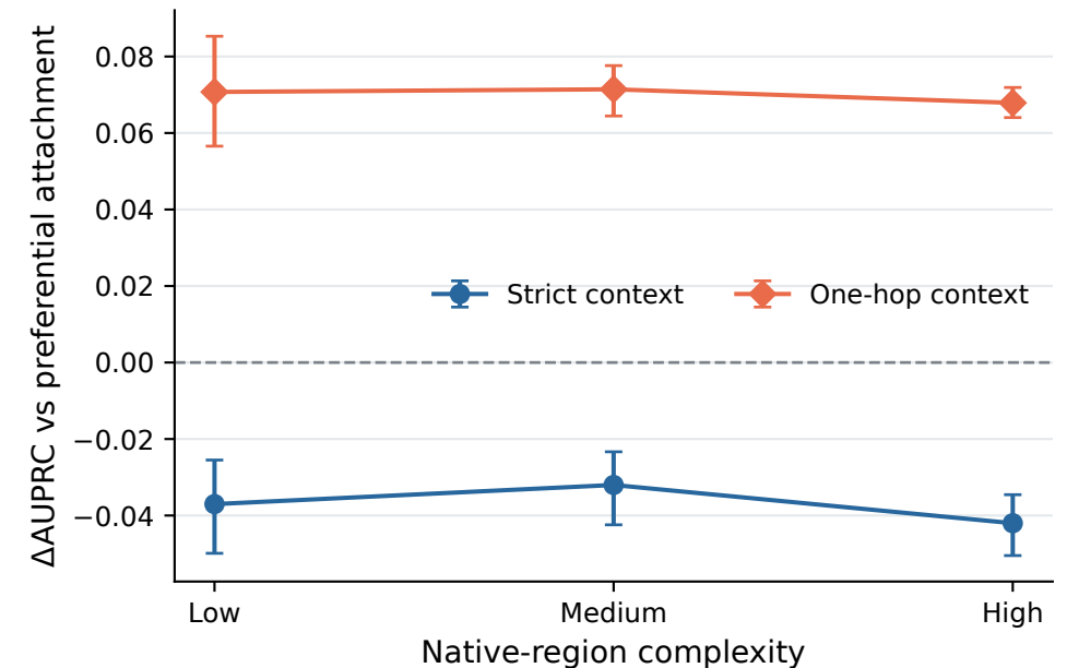
b Context effect across native-region complexity
