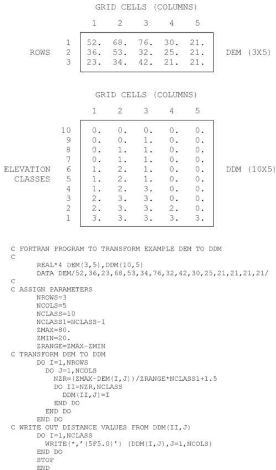
Figure 8. The relationship between a DEM and an extracted DDM is presented using a small example data set. The FORTRAN code used to create the 10 x 5 DDM from the 3 x 5 DEM is listed below the diagrams.
