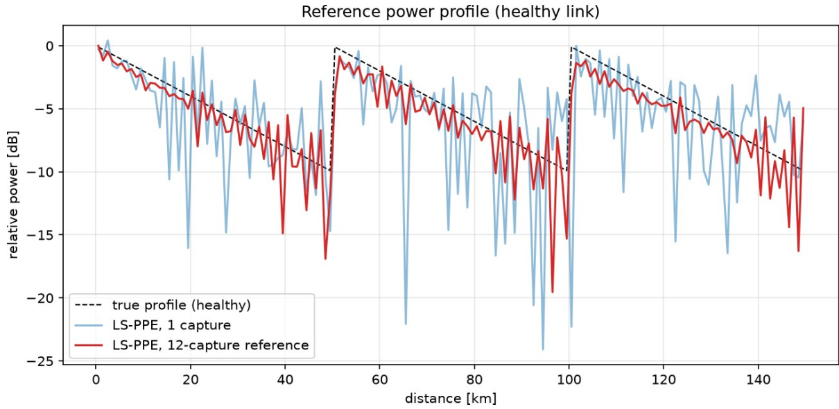
Fig. 1 Healthy-link power profile: single-capture LS-PPE (blue) is visibly noisy; the 12-capture average (red) serves as the reference, with the three-span sawtooth structure clearly resolved.
