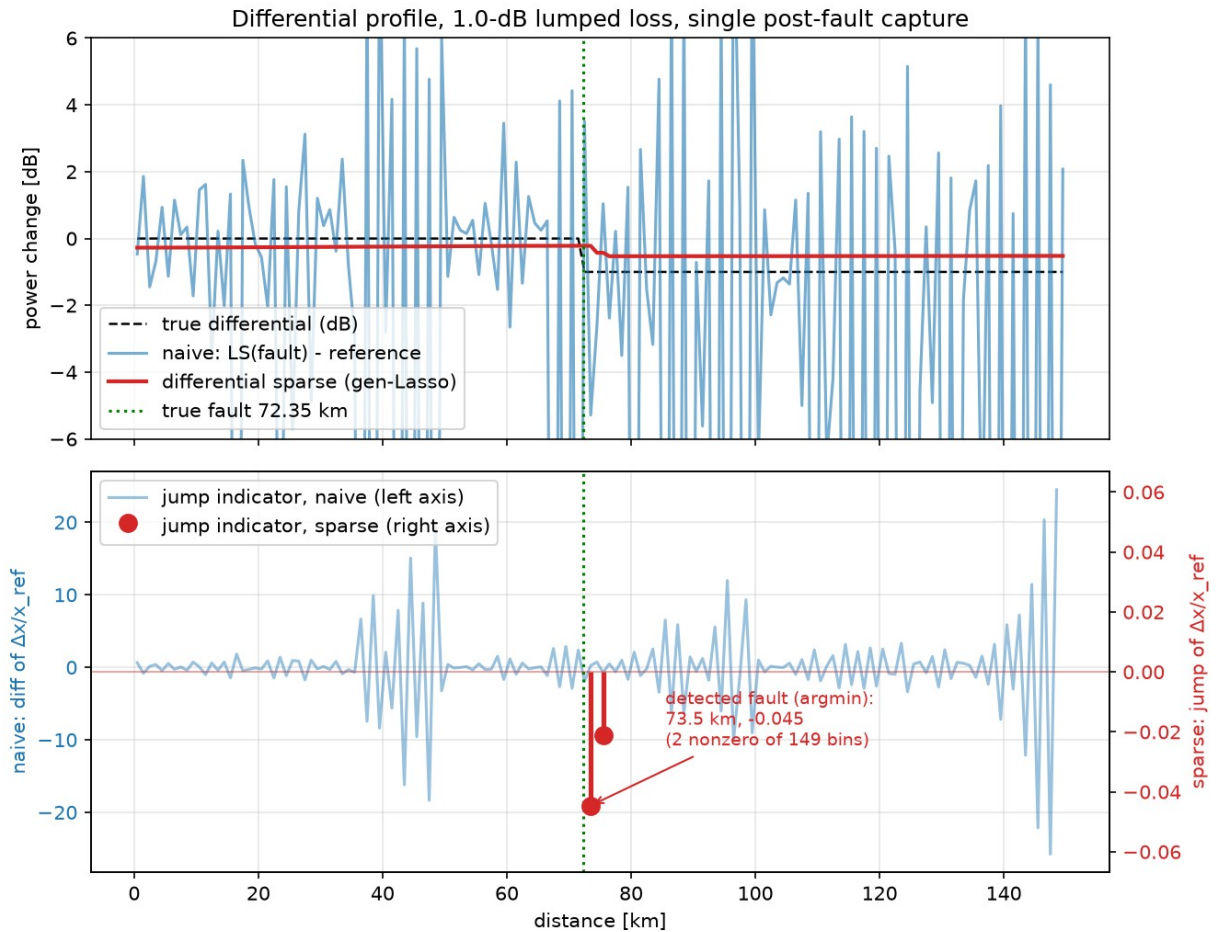
Fig. 2 1-dB lumped loss, single post-fault capture. Top: naive subtraction (blue) is buried in noise, while the differential sparse solution (red) is a clean step at the right position (amplitude shrunk by the Lasso; refit in Sec. 5.3).
