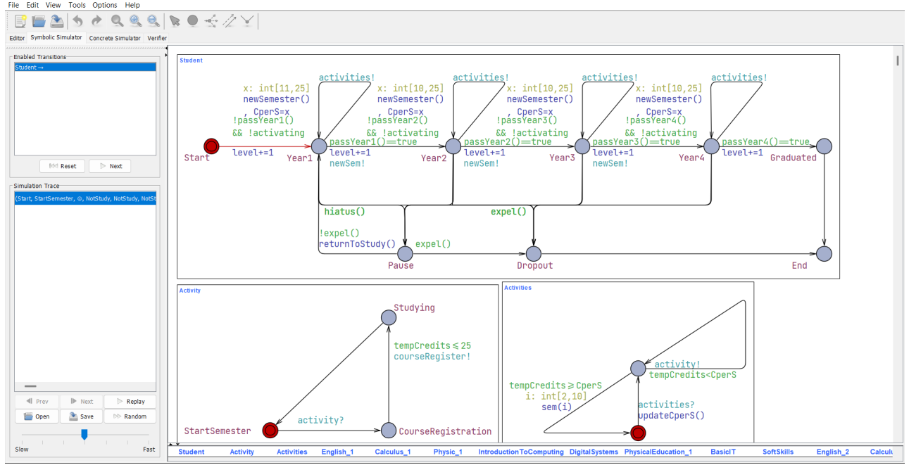
Figure 2: UPPAAL implementation of the student lifecycle model.
