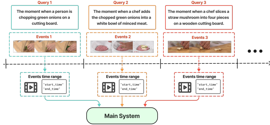
Fig. 3: Progressive Event Filtering Mechanism. Each query ( Q1 , Q2 , Q3 ) retrieves the top-matched events from the video, represented as 10-second segments with 2-second overlap. The corresponding temporal intervals ( start\_time , end\_time ) are then converted into constraints that define valid search regions. When subsequent queries are added, the filter dynamically updates to include only events that are both semantically relevant and temporally consecutive to previous results. These refined intervals are passed to the main retrieval system, ensuring coherent and temporally consistent event linking.
