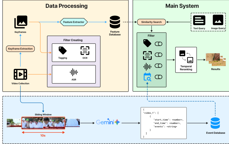
Fig. 1: System pipeline showing multimodal filtering and event-based retrieval. The filter module integrates Tagging, OCR, ASR, and Event Capturing to generate temporal constraints that refine similarity search and ensure coherent, context-aware results.
