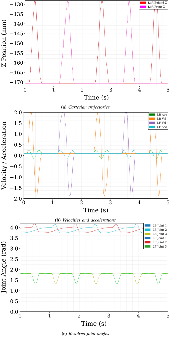
Fig. 3: Left front limb gait trajectory mapping
