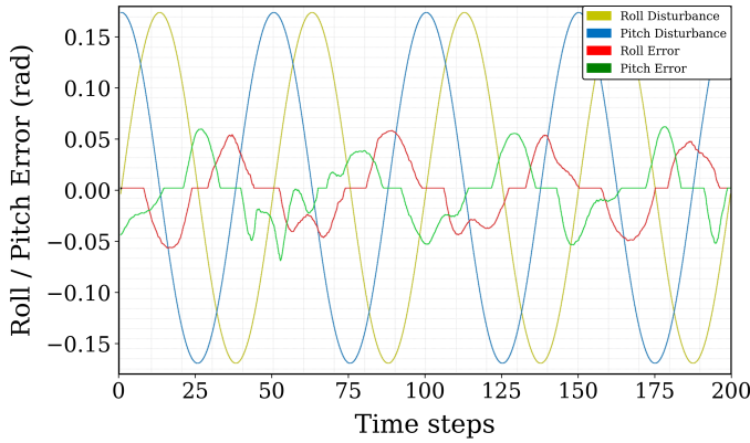
Fig. 6: Controller error response during dynamic trotting gait
