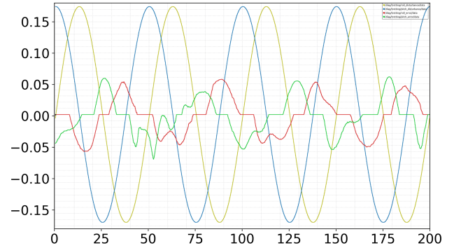
Fig. 5: Controller error response during dynamic trotting gait
