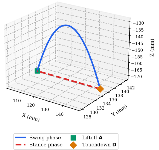
Fig. 2: 3D foot trajectory for the left front limb
