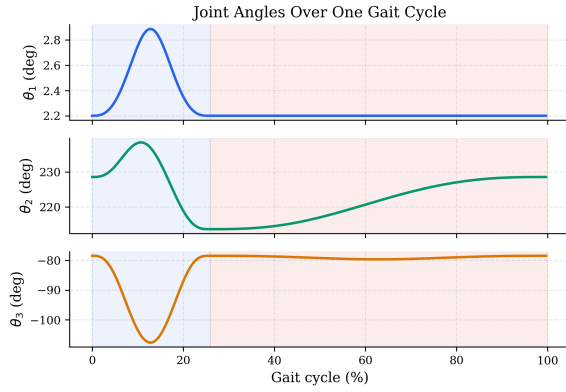
(b) Resolved joint angles for the left front limb.
