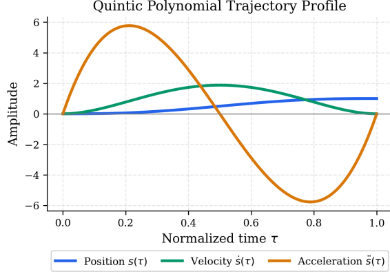
(a) Quintic polynomial PVA profiles.
