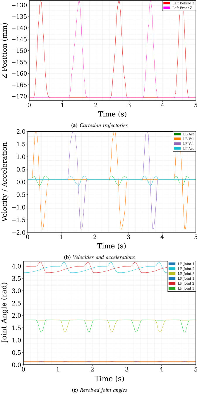
Fig. 3: Simulation mapping for the left front limb tracking one complete gait cycle
