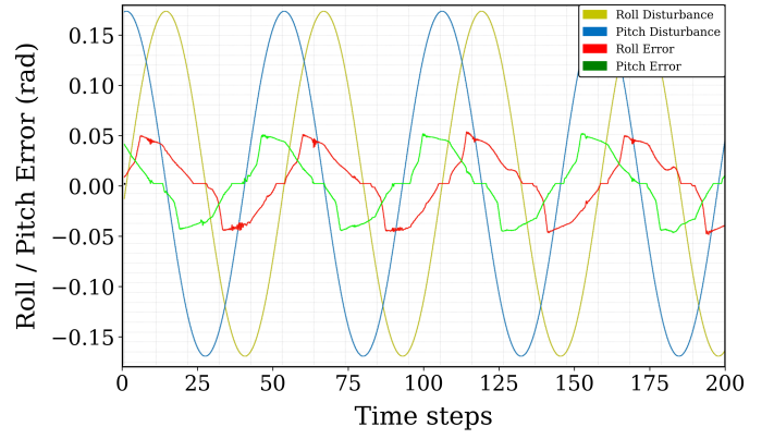
Fig. 4: Controller error response during static home posture
