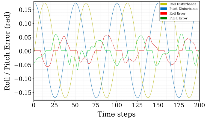
Fig. 5: Controller error response during dynamic trotting gait
