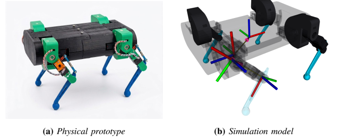
Fig. 1: Quadruped robot physical prototype and simulation model with reference frames
