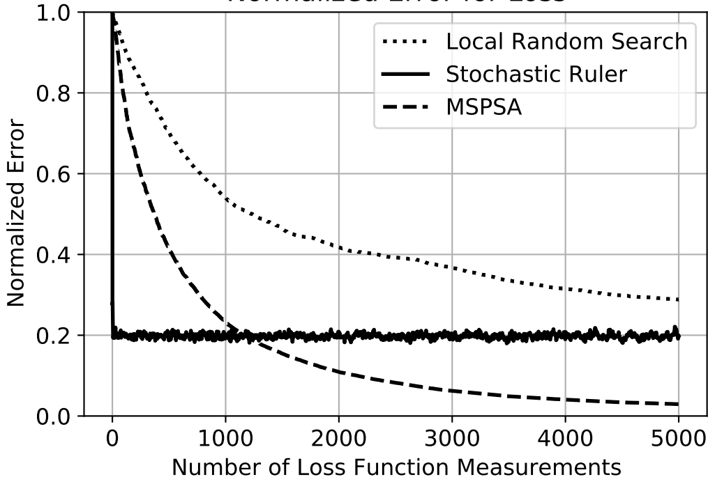
Normalized Error for Loss
