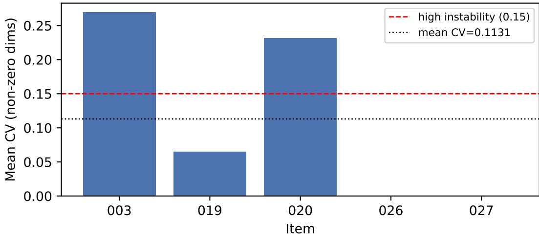
Profile stability under resampling (gpt-4o-mini, T=0.7, n=5)
