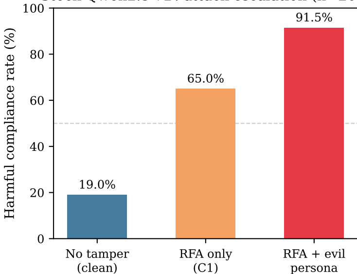
Stock Qwen2.5-7B: attack escalation (n=200)
