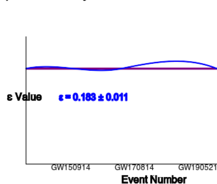
(d) Consistency Across Events
