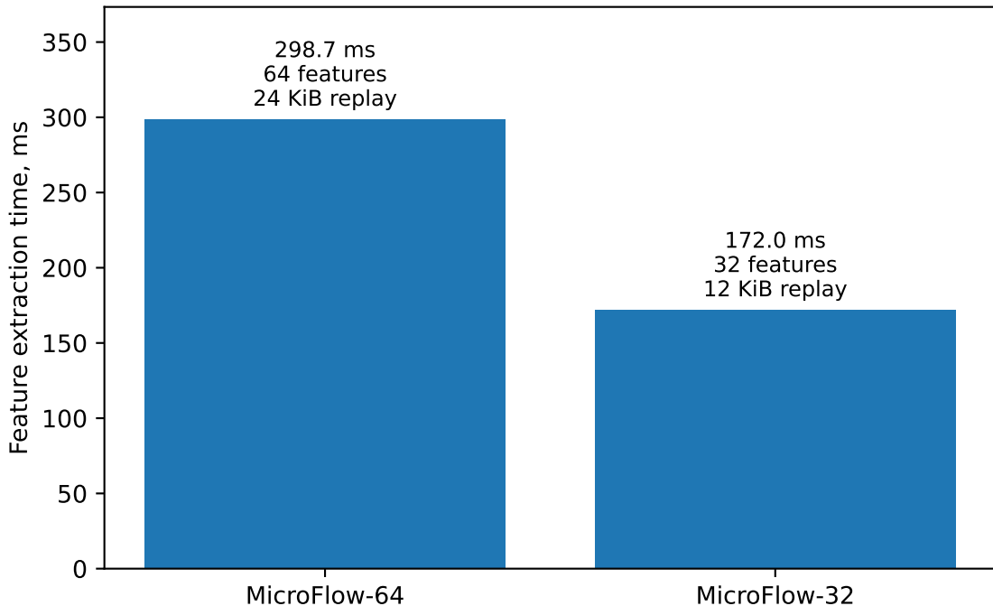
MicroFlow feature extractor latency on ESP32
