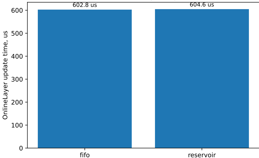
Device-side RAM-only CL update cost
