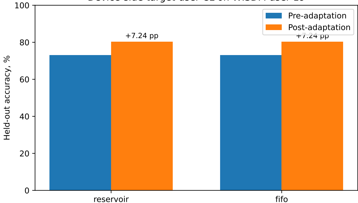
Device-side target-user CL on WISDM user 19
