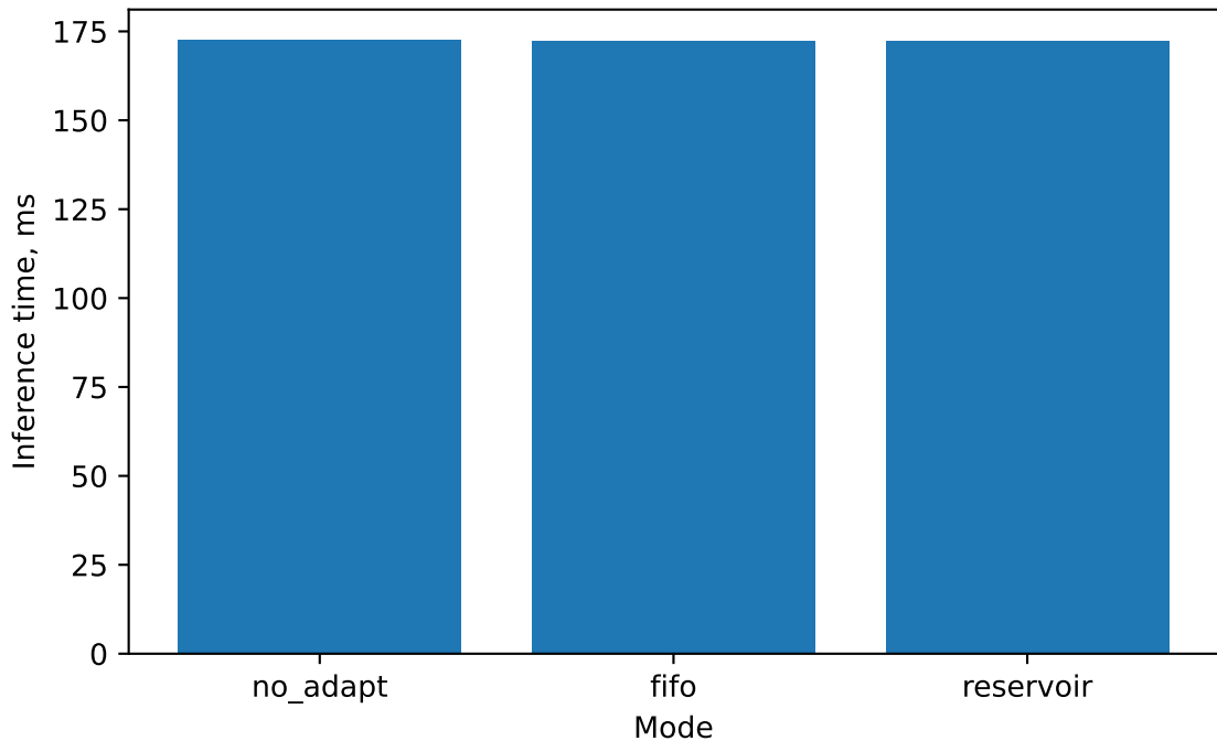
MicroFlow-32 inference latency on ESP32
